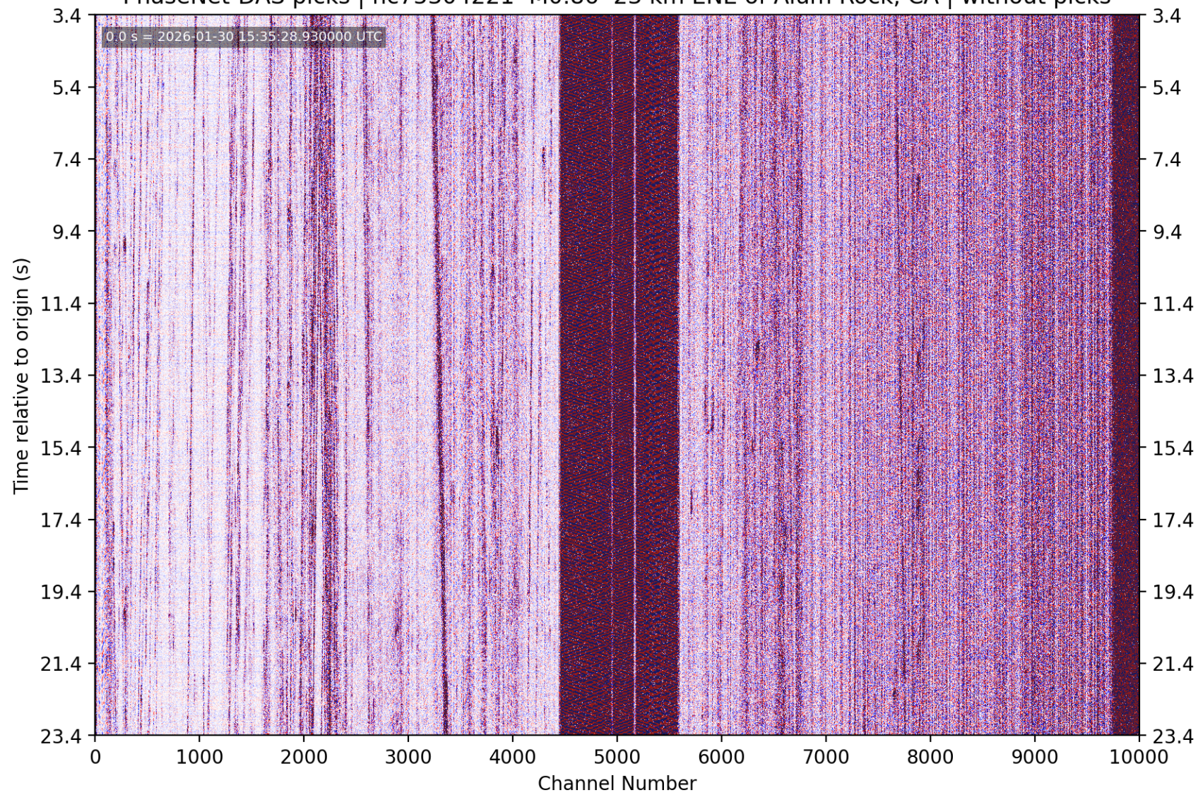
PhaseNet-DAS picks | nc75304221 M0.86 23 km ENE of Alum Rock, CA | without picks
