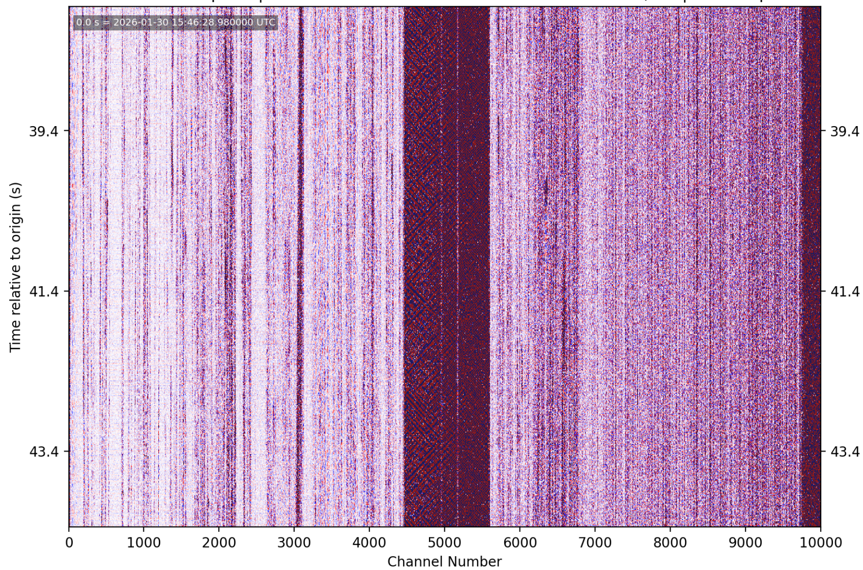
PhaseNet-DAS picks | nc75304236 M0.98 23 km ENE of Alum Rock, CA | without picks
