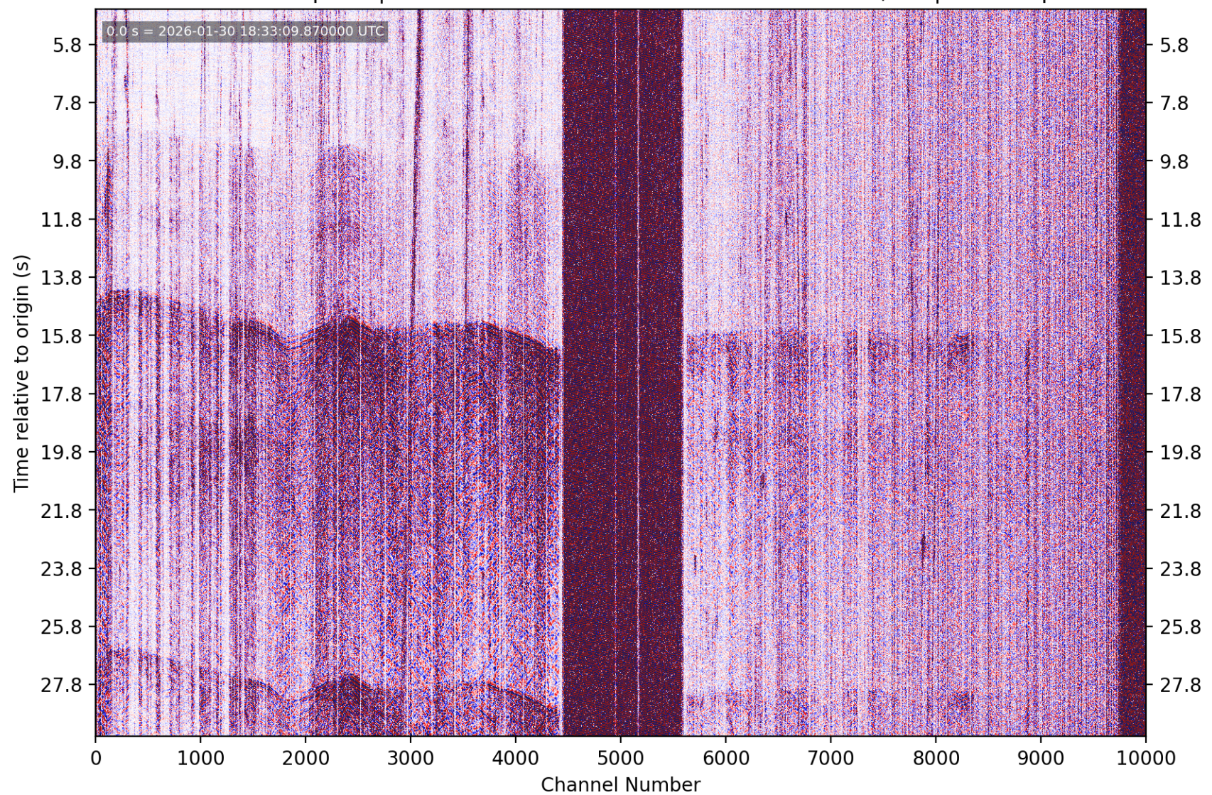
PhaseNet-DAS picks | nc75304291 M3.4 4 km SE of San Ramon, CA | without picks
