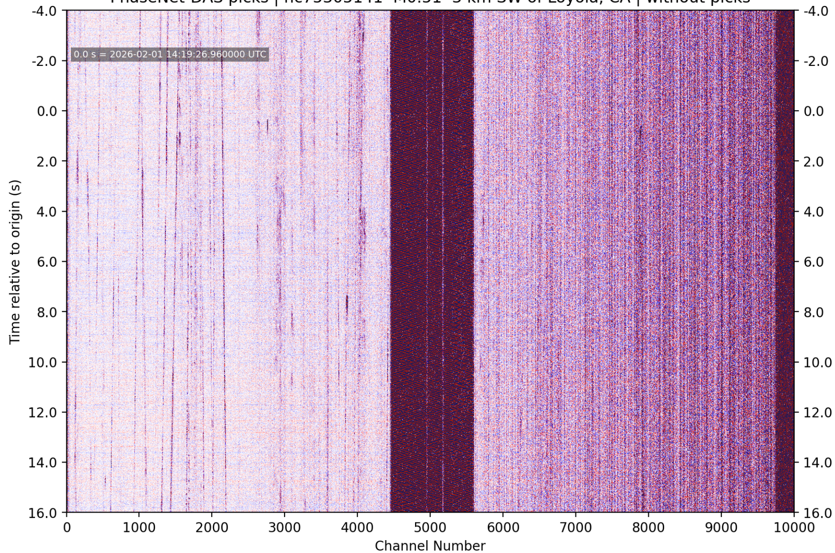
PhaseNet-DAS picks | nc75305141 M0.51 3 km SW of Loyola, CA | without picks
