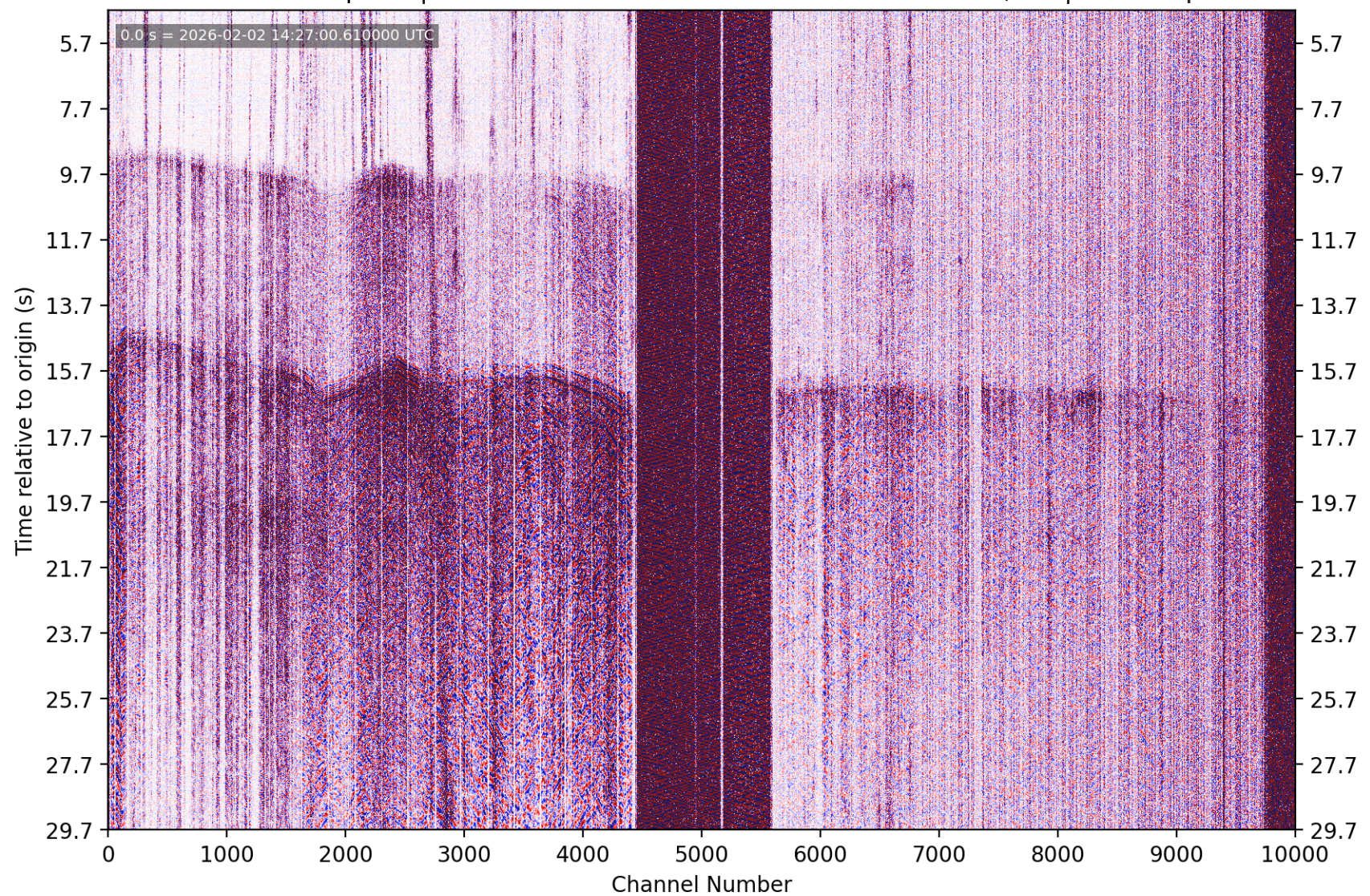
PhaseNet-DAS picks | nc75305671 M3.8 4 km SSE of San Ramon, CA | without picks
