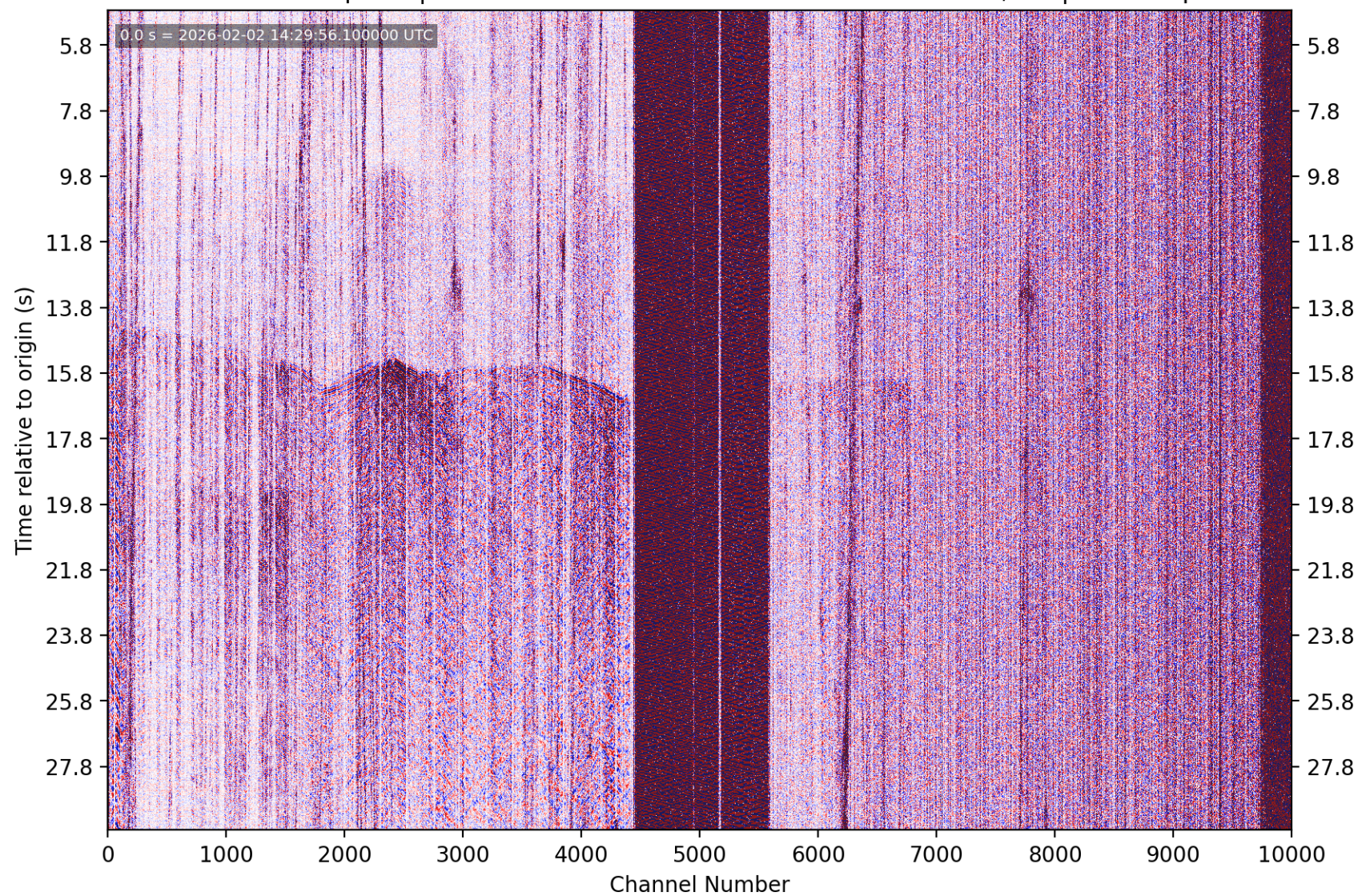
PhaseNet-DAS picks | nc75305676 M3.13 4 km SE of San Ramon, CA | without picks
