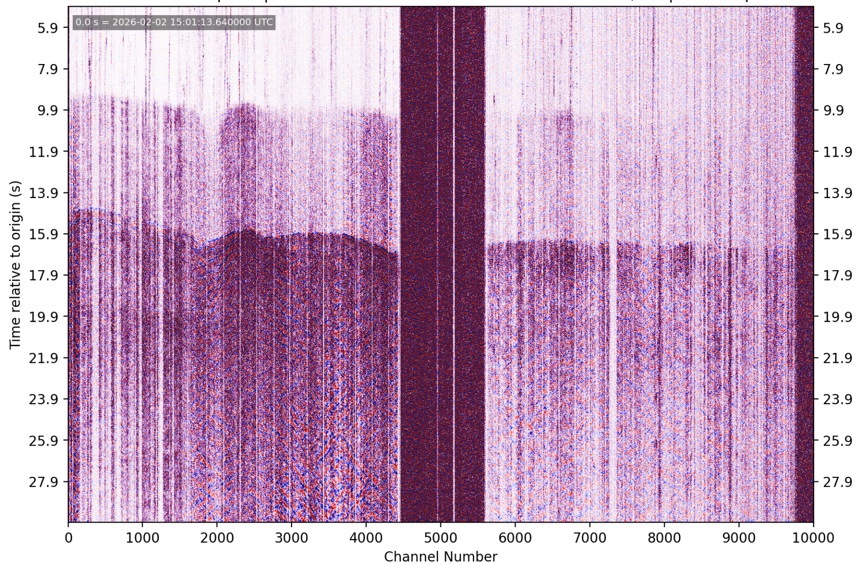
PhaseNet-DAS picks | nc75305736 M4.18 4 km SE of San Ramon, CA | without picks
