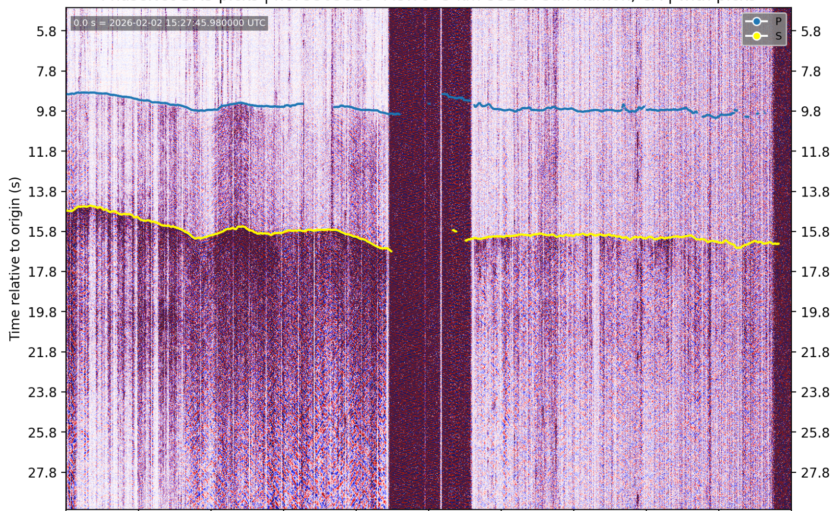
PhaseNet-DAS picks | nc75305826 M3.79 5 km SSE of San Ramon, CA | without picks
