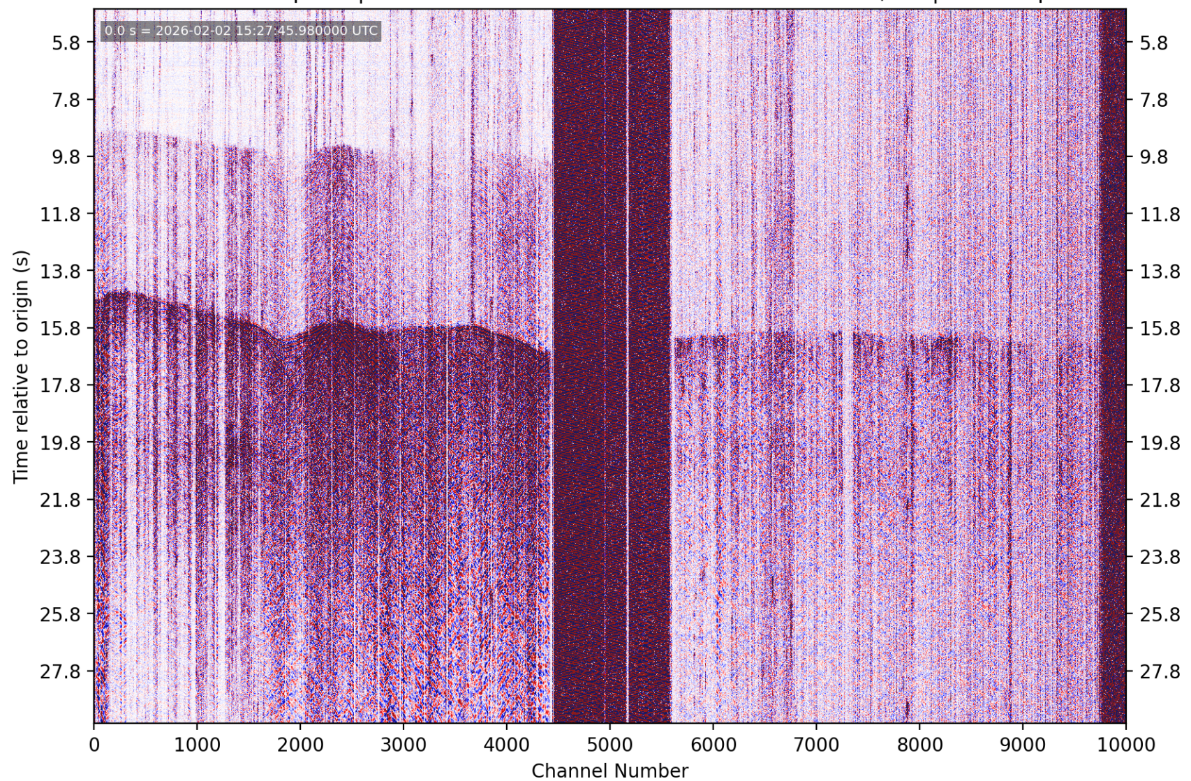
PhaseNet-DAS picks | nc75305826 M3.79 5 km SSE of San Ramon, CA | without picks
