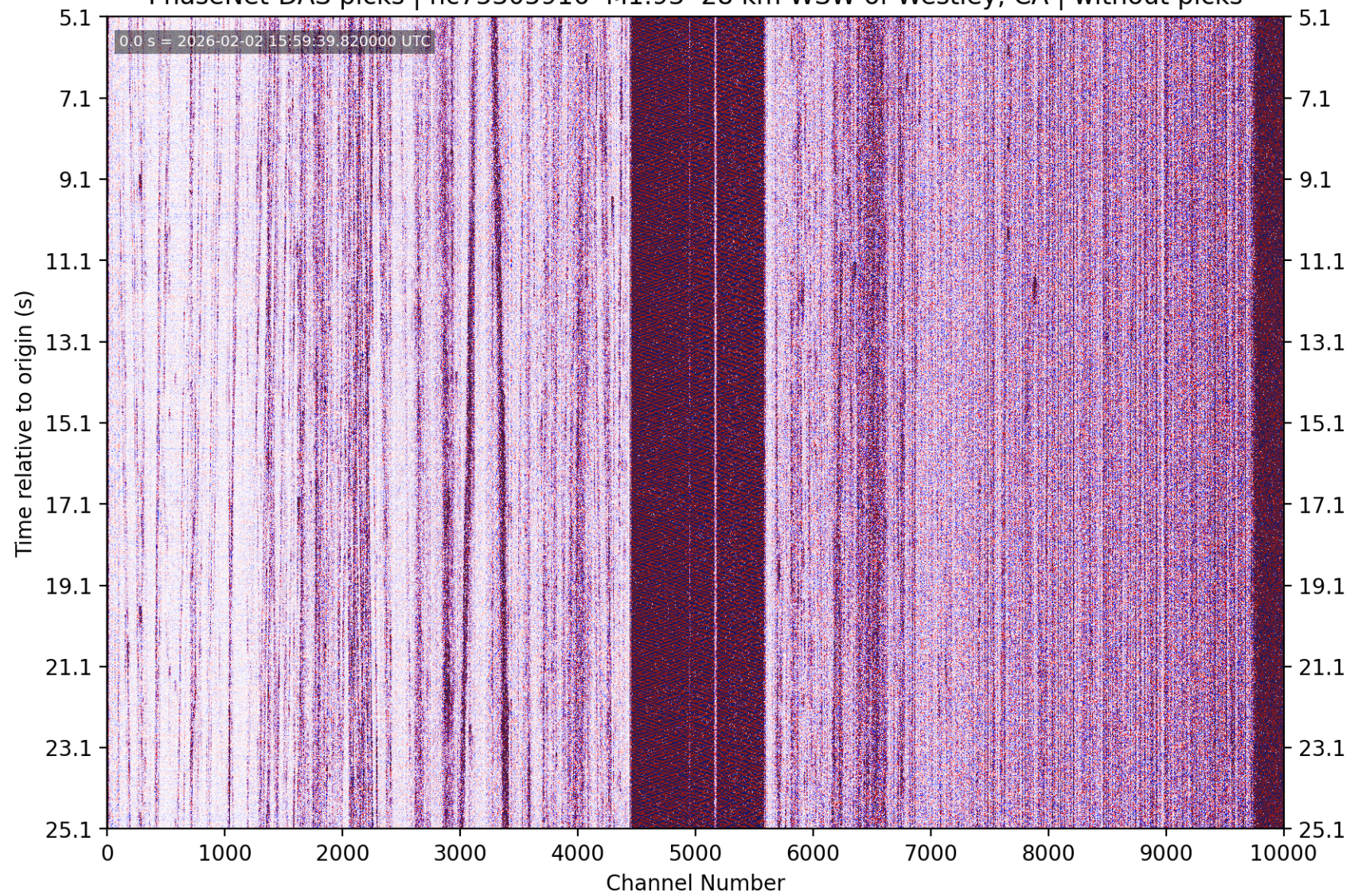
PhaseNet-DAS picks | nc75305916 M1.93 28 km WSW of Westley, CA | without picks
