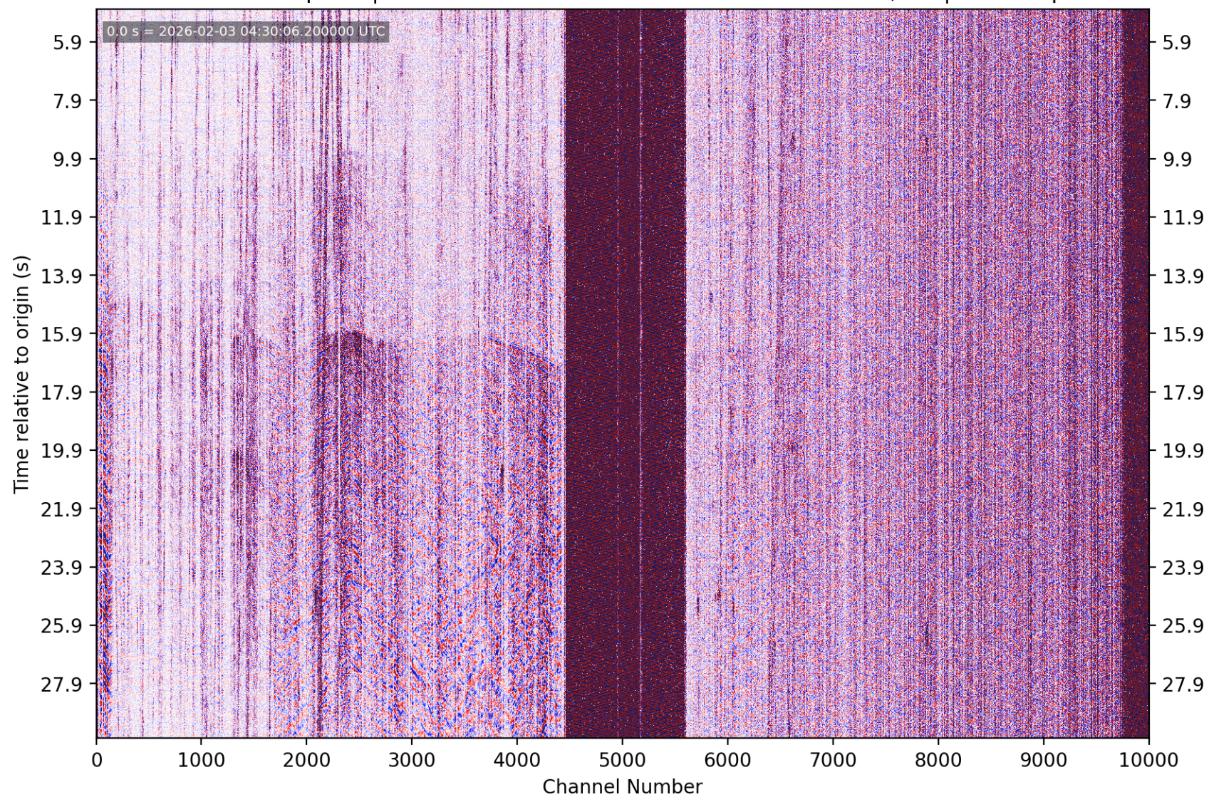
PhaseNet-DAS picks | nc75306461 M3.24 5 km SE of San Ramon, CA | without picks
