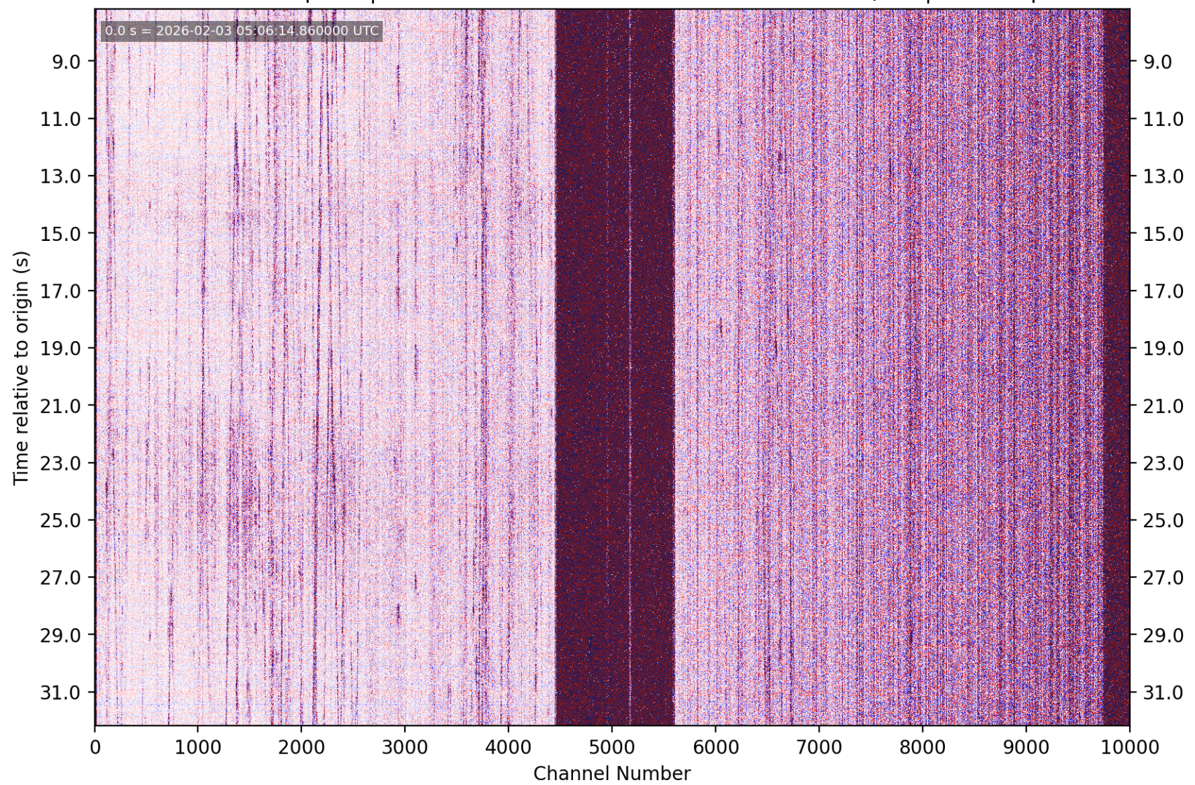
PhaseNet-DAS picks | nc75306486 M2.12 8 km NE of Alum Rock, CA | without picks
