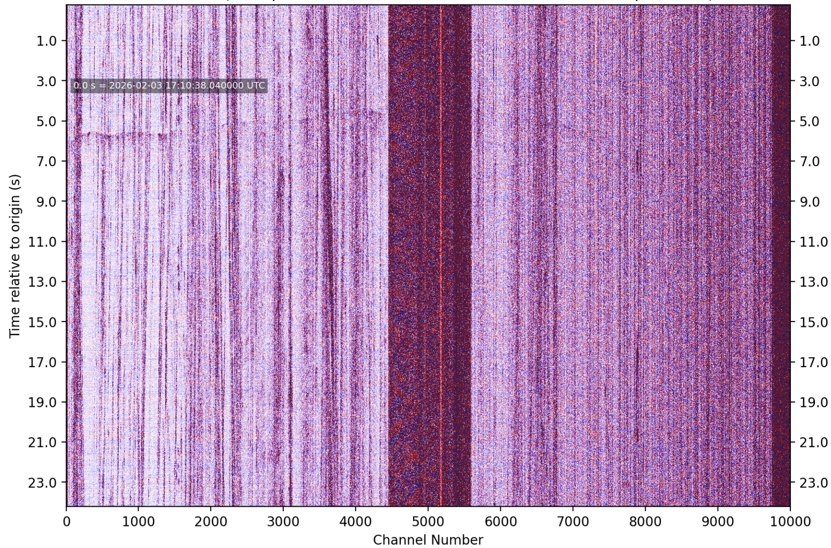
PhaseNet-DAS picks | nc75306801 M1.01 3 km SE of Pacifica, CA | without picks
