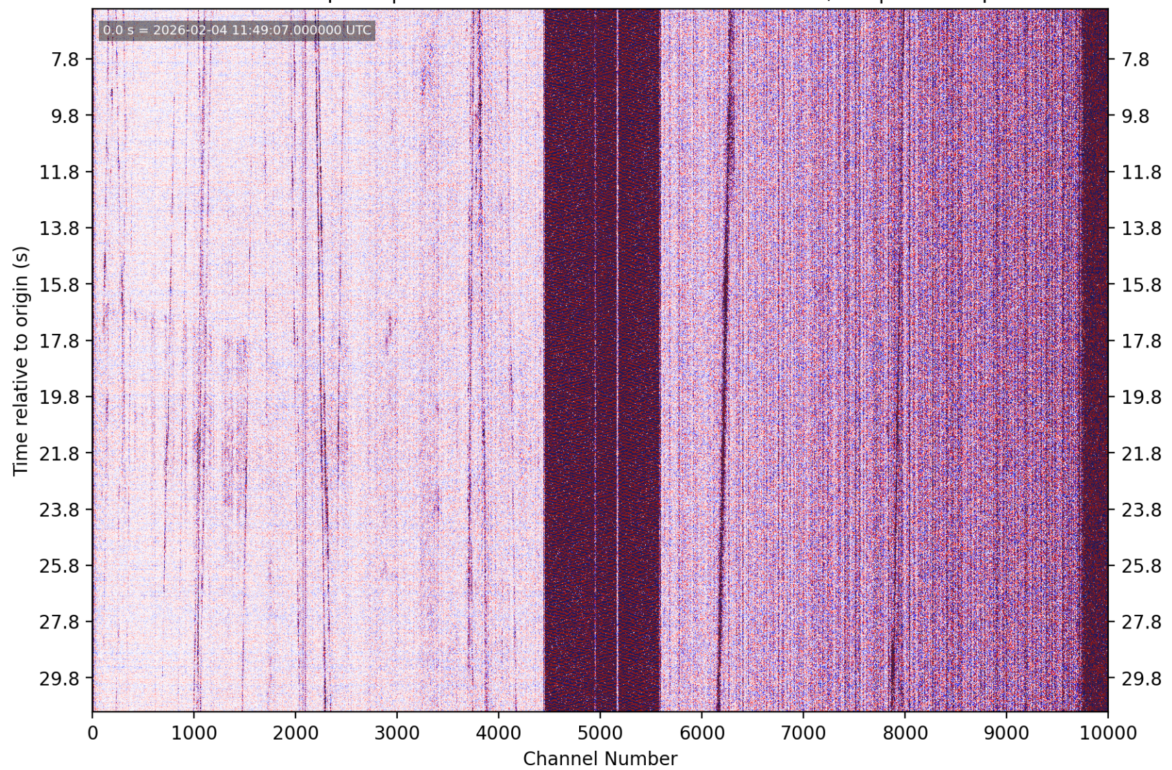
PhaseNet-DAS picks | nc75308267 M1.99 6 km SE of Sunol, CA | without picks
