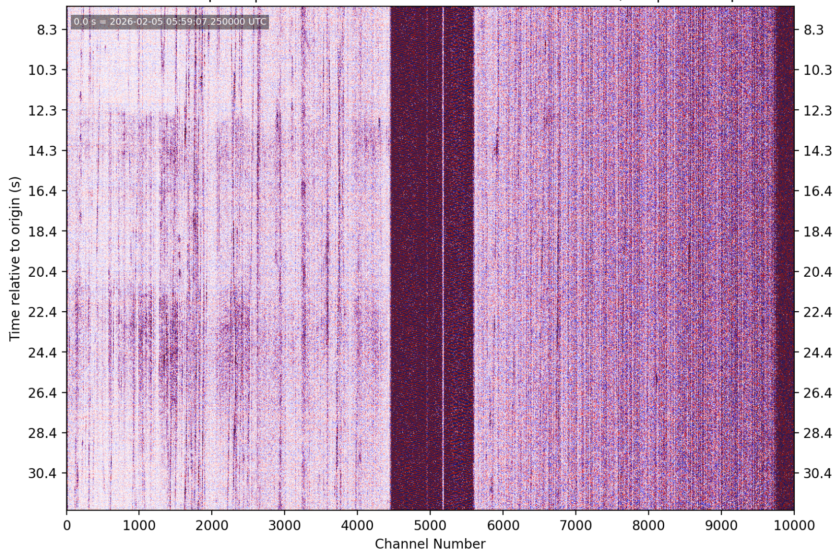
PhaseNet-DAS picks | nc75308762 M2.27 5 km NNE of Alum Rock, CA | without picks
