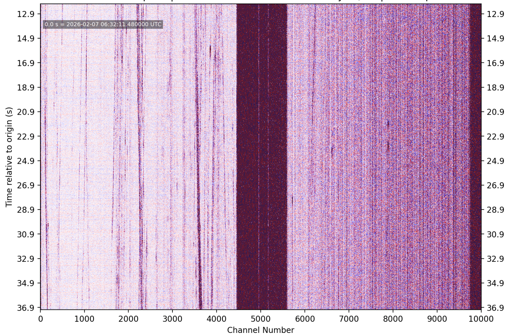
PhaseNet-DAS picks | nc75309947 M1.15 6 km S of Loyola, CA | without picks
