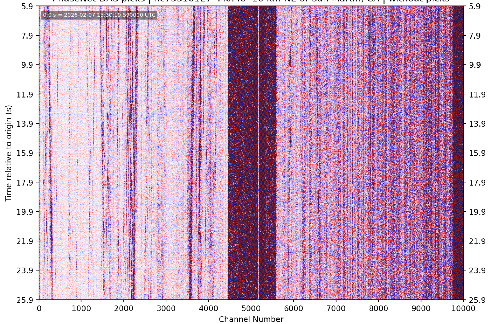
PhaseNet-DAS picks | nc75310127 M0.48 10 km NE of San Martin, CA | without picks
