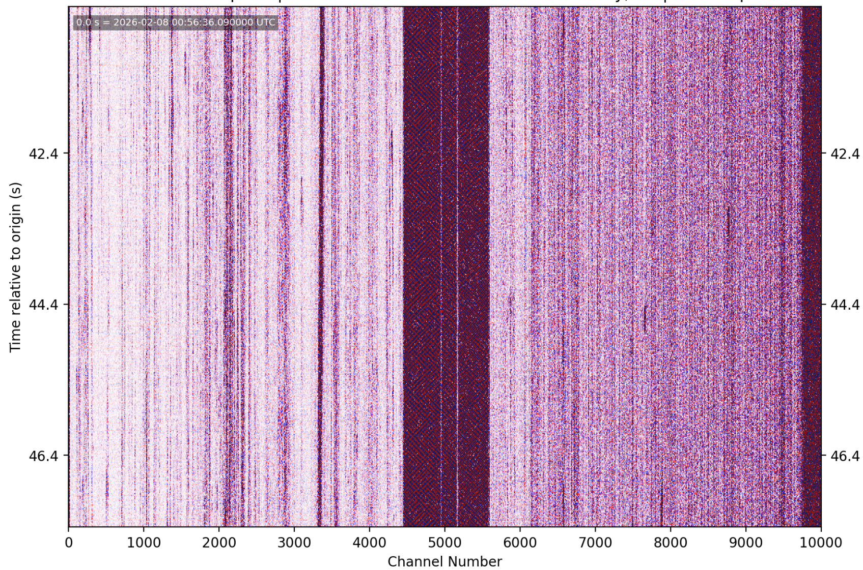
PhaseNet-DAS picks | nc75310367 M0.92 7 km WSW of Gilroy, CA | without picks
