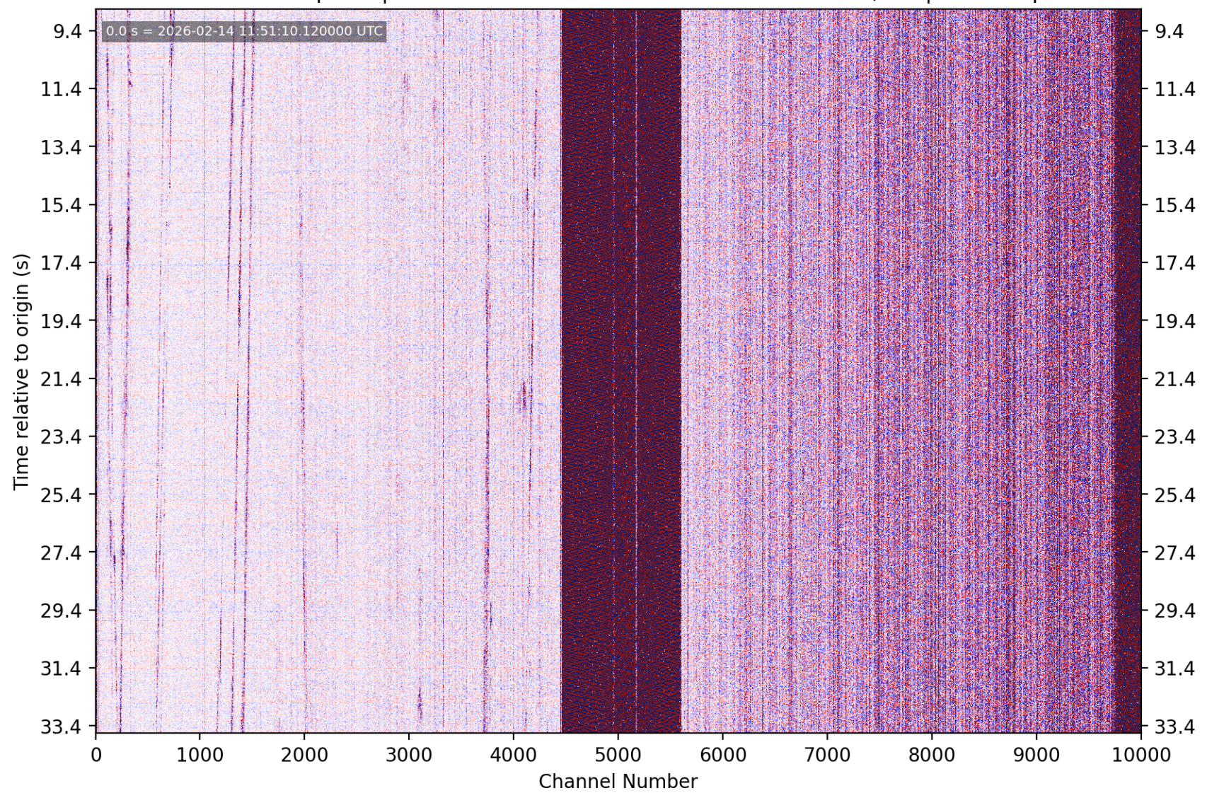
PhaseNet-DAS picks | nc75313672 M1.18 8 km E of Alum Rock, CA | without picks
