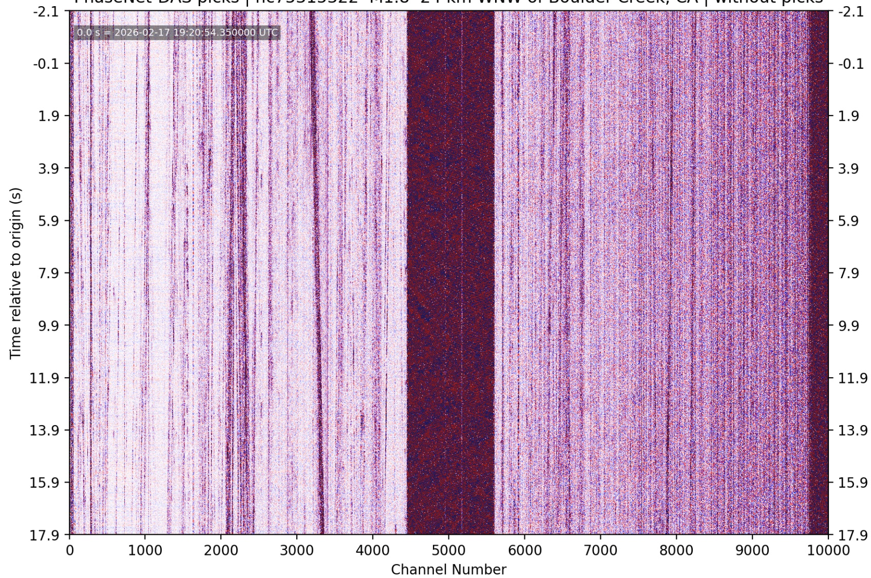
PhaseNet-DAS picks | nc75315322 M1.8 24 km WNW of Boulder Creek, CA | without picks
