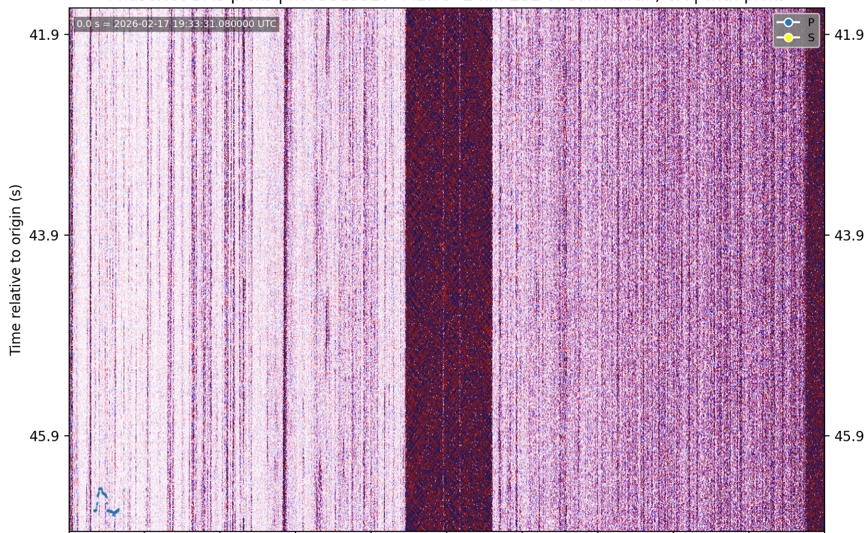
PhaseNet-DAS picks | nc75315327 M2.73 2 km ESE of San Martin, CA | without picks
