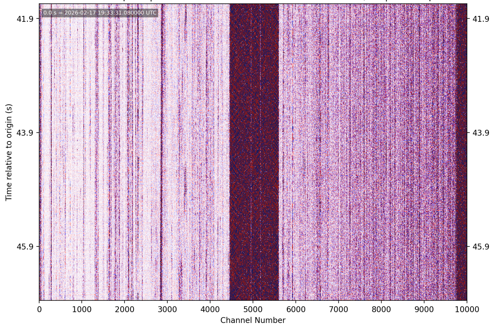
PhaseNet-DAS picks | nc75315327 M2.73 2 km ESE of San Martin, CA | without picks
