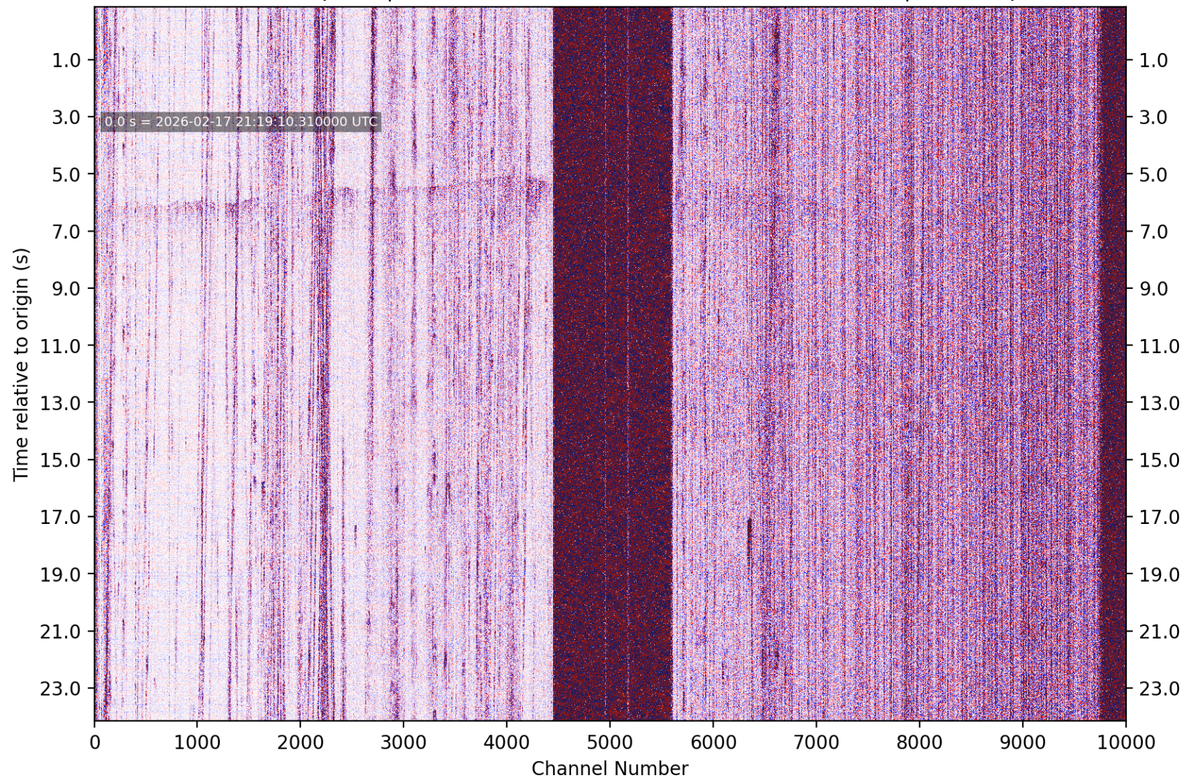
PhaseNet-DAS picks | nc75315362 M1.32 3 km SE of Pacifica, CA | without picks
