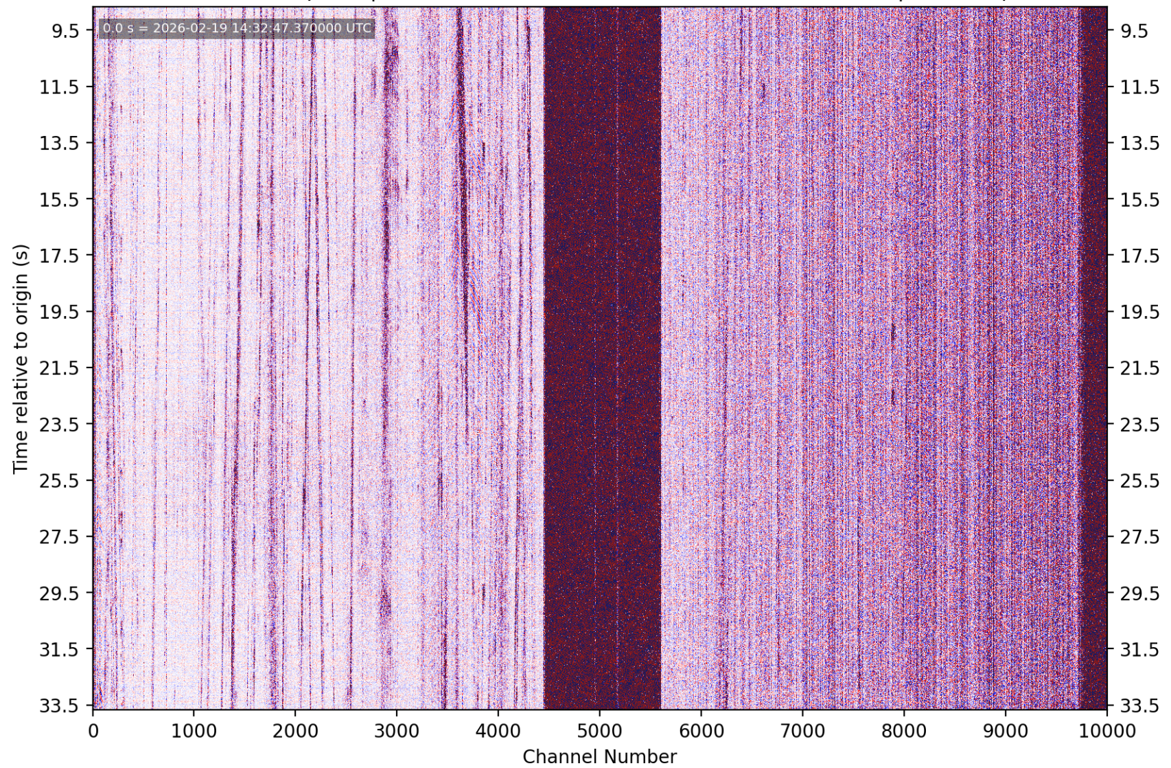
PhaseNet-DAS picks | nc75315867 M1.85 9 km E of Alum Rock, CA | without picks
