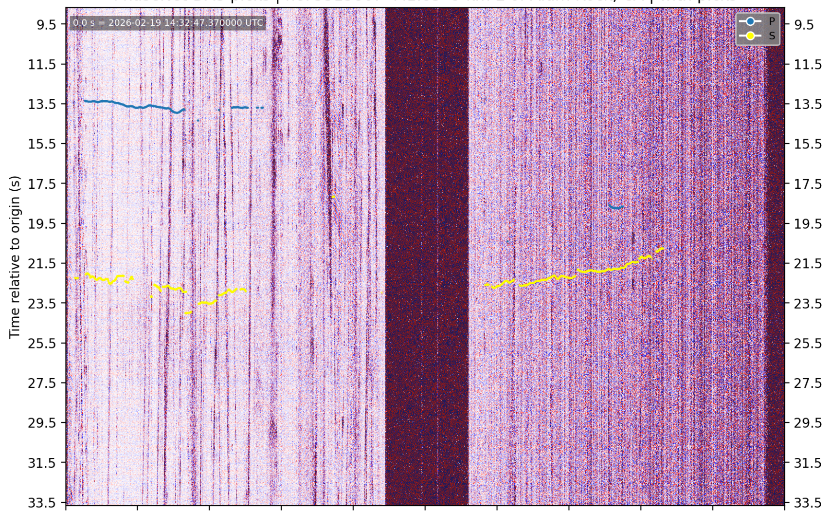
PhaseNet-DAS picks | nc75315867 M1.85 9 km E of Alum Rock, CA | without picks
