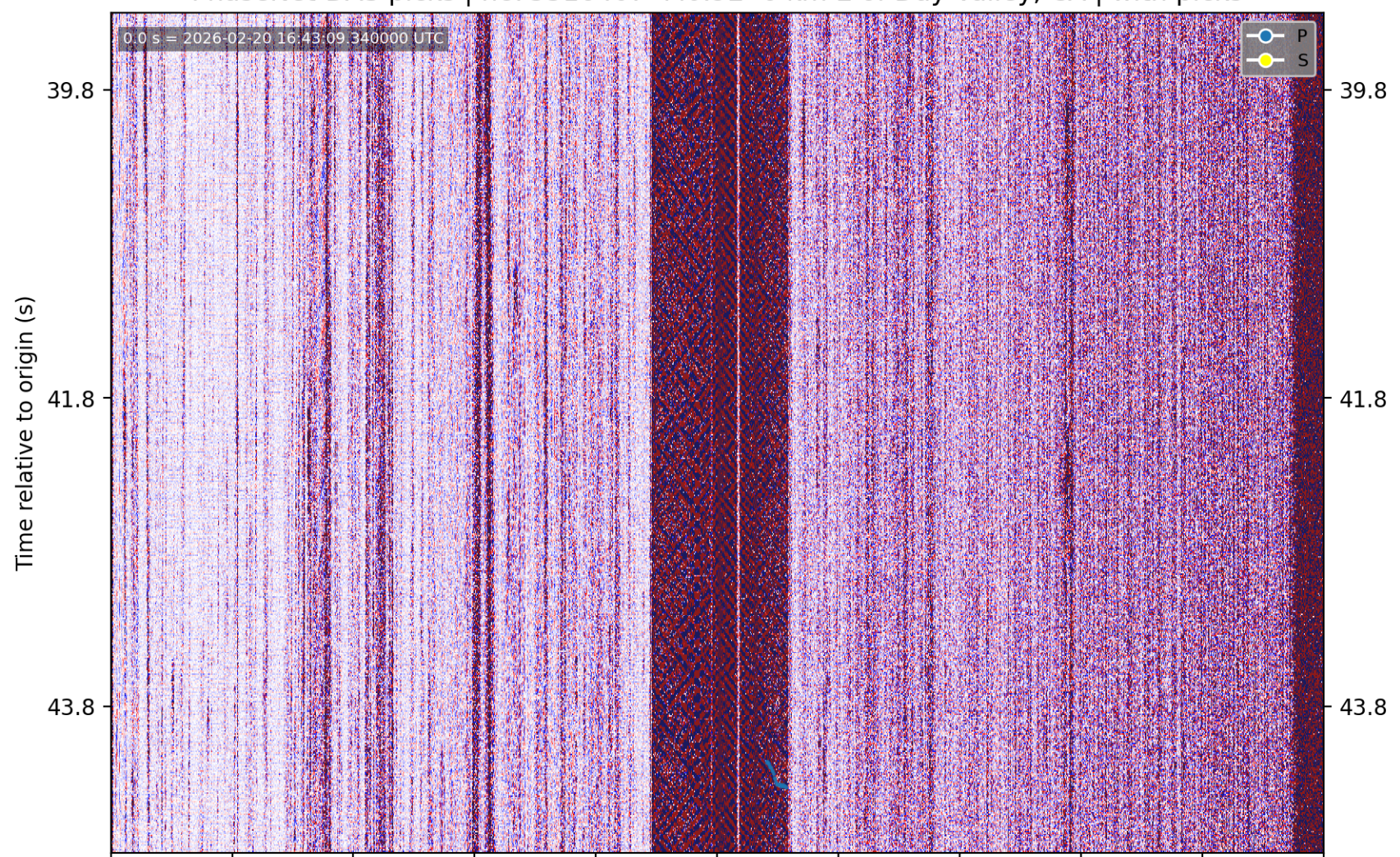
PhaseNet-DAS picks | nc75316407 M0.92 6 km E of Day Valley, CA | without picks
