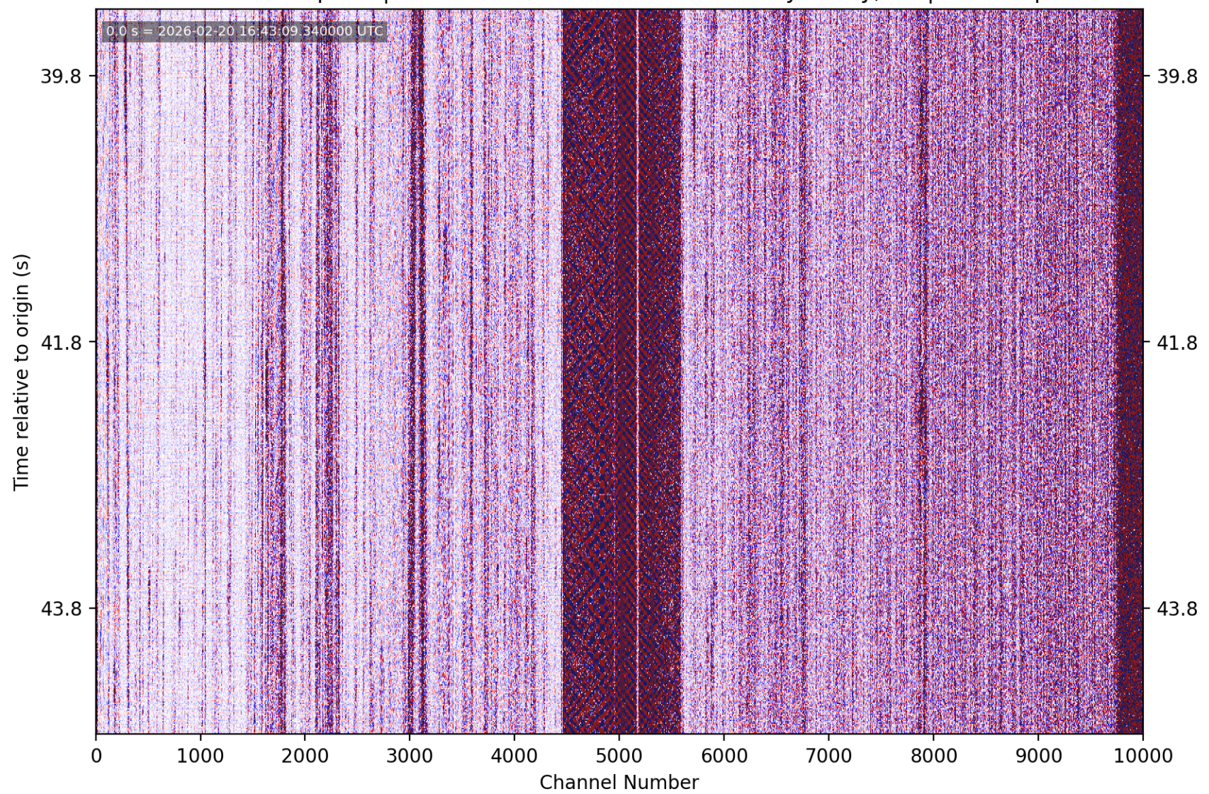
PhaseNet-DAS picks | nc75316407 M0.92 6 km E of Day Valley, CA | without picks
