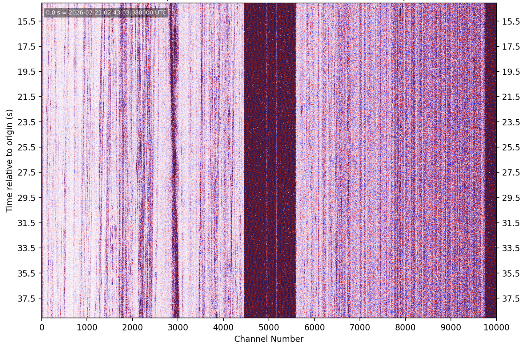
PhaseNet-DAS picks | nc75316567 M1.83 9 km E of Alum Rock, CA | without picks
