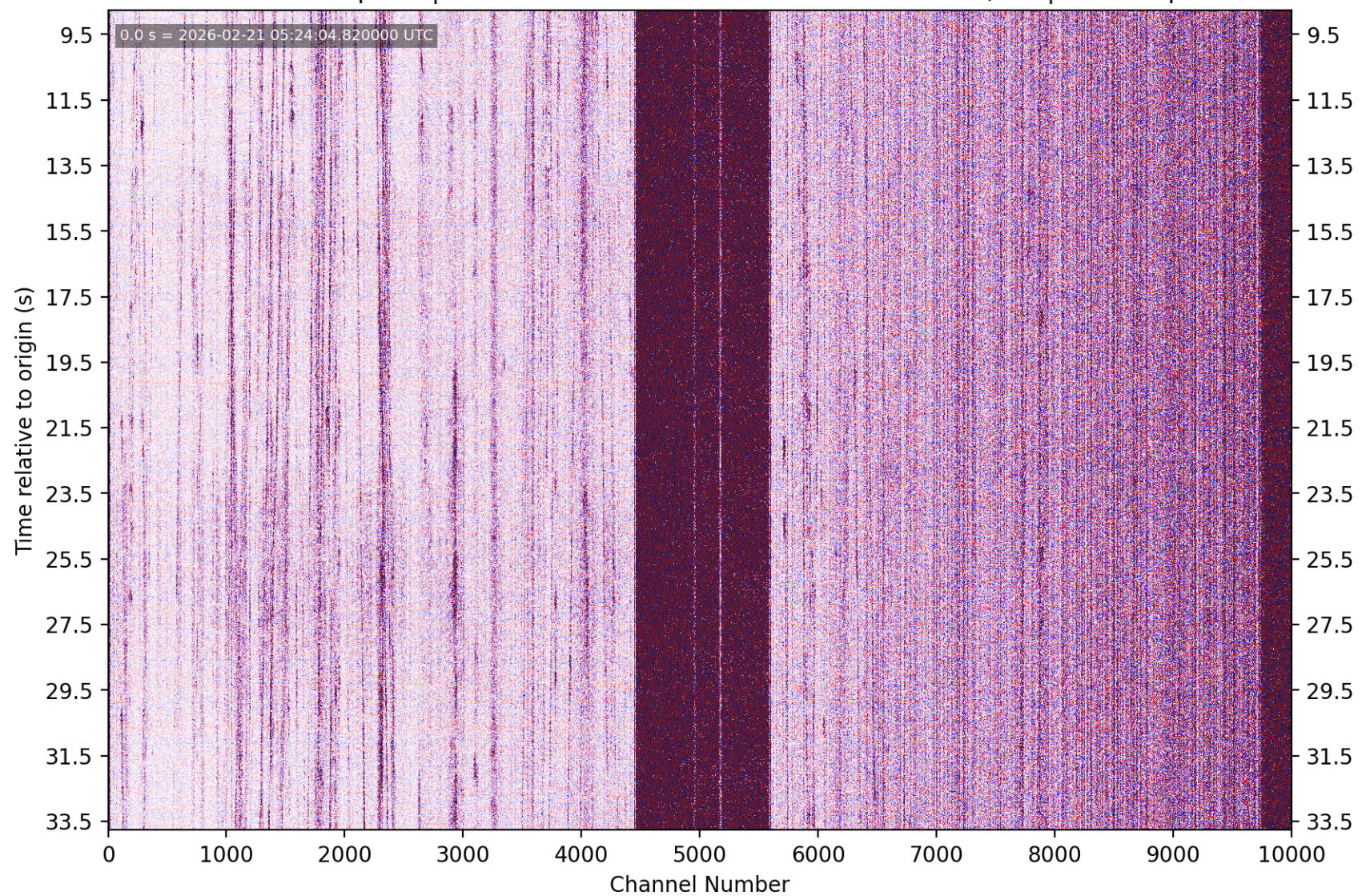
PhaseNet-DAS picks | nc75316587 M2.18 9 km E of Alum Rock, CA | without picks
