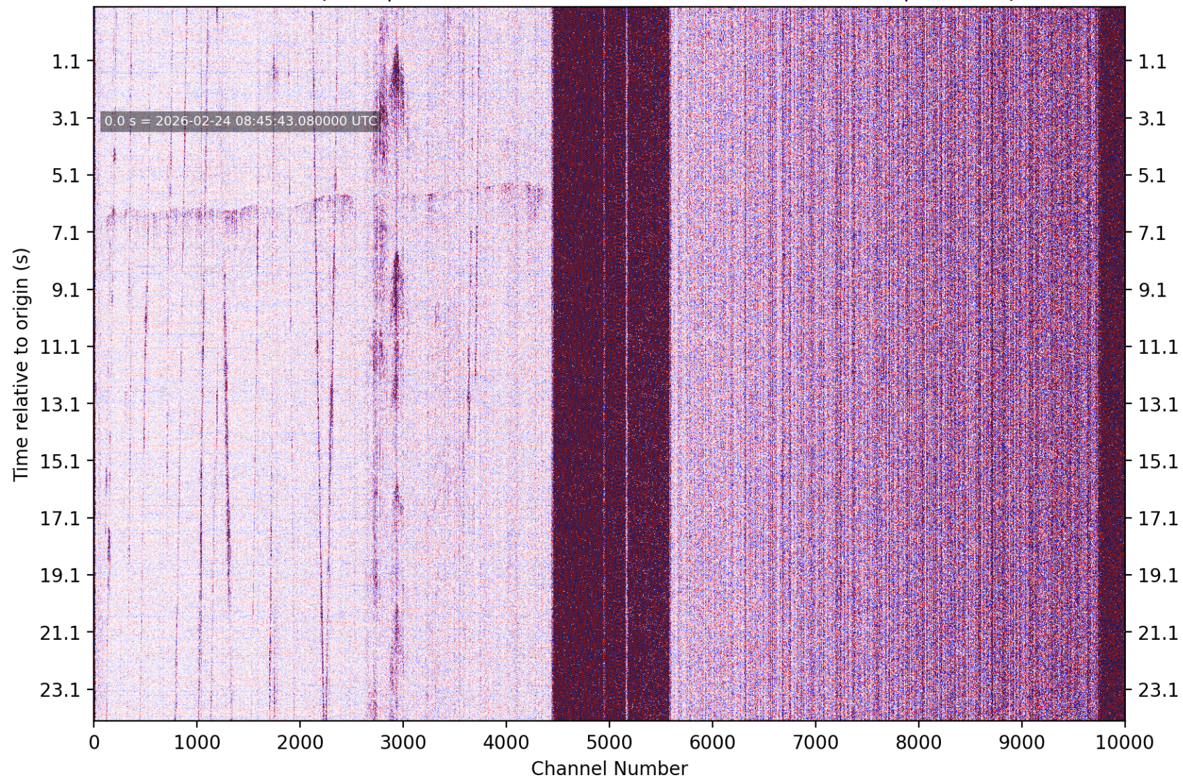
PhaseNet-DAS picks | nc75318332 M1.13 3 km SE of Pacifica, CA | without picks
