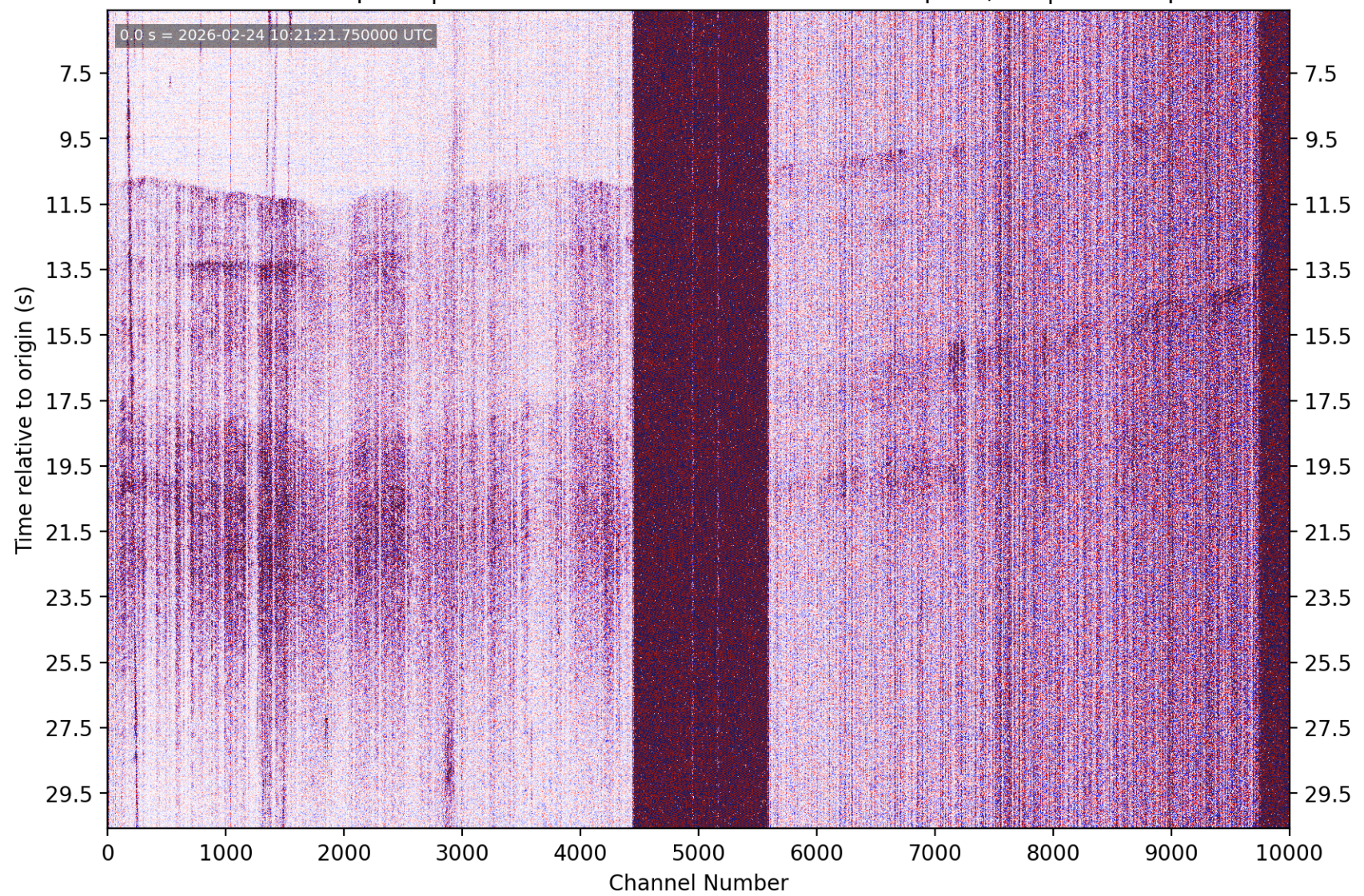
PhaseNet-DAS picks | nc75318362 M2.52 9 km NNE of Milpitas, CA | without picks
