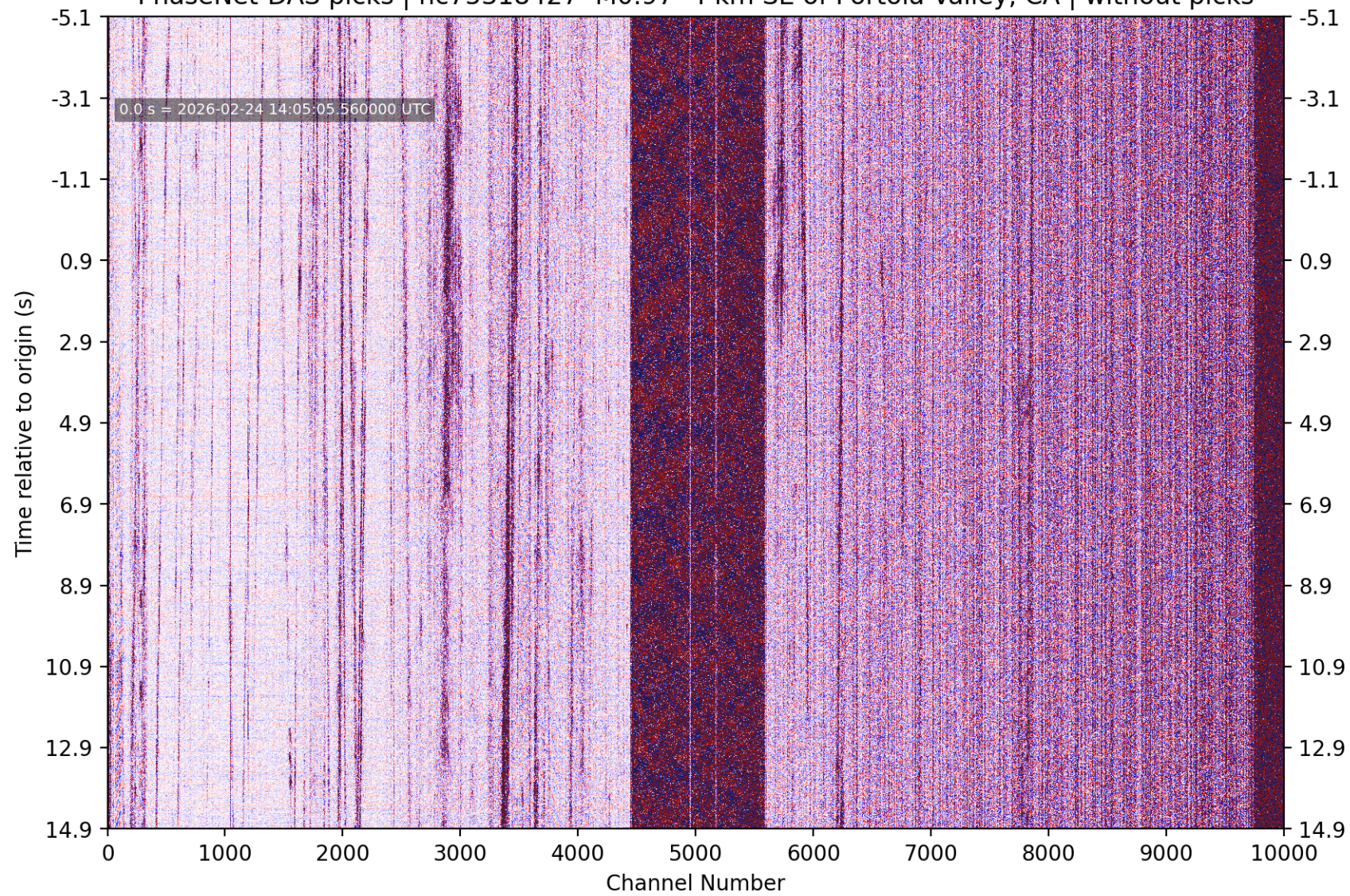
PhaseNet-DAS picks | nc75318427 M0.97 4 km SE of Portola Valley, CA | without picks
