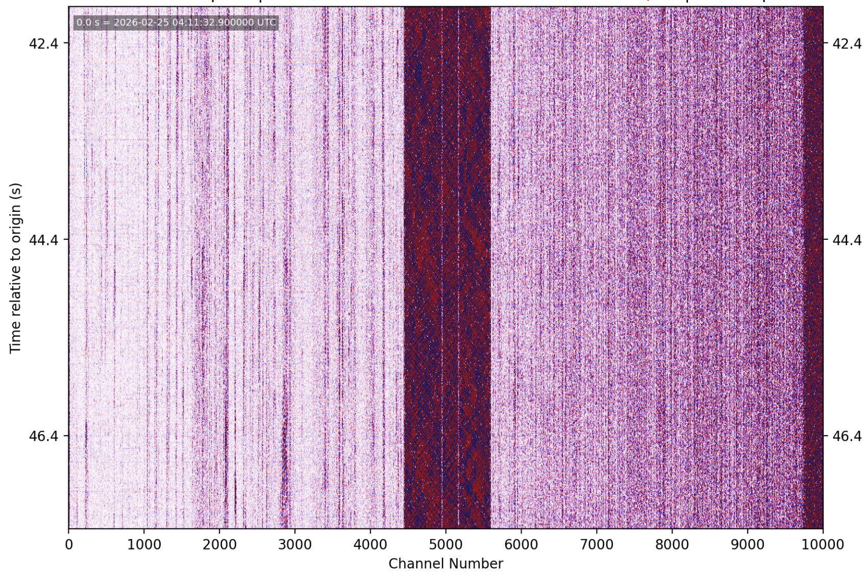
PhaseNet-DAS picks | nc75318652 M0.98 11 km ENE of San Martin, CA | without picks
