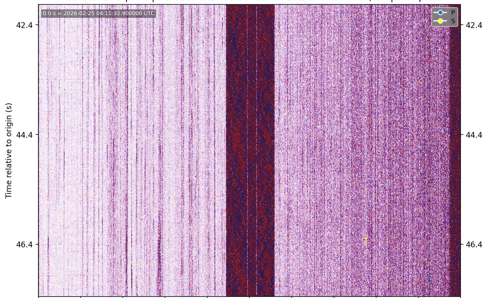
PhaseNet-DAS picks | nc75318652 M0.98 11 km ENE of San Martin, CA | without picks
