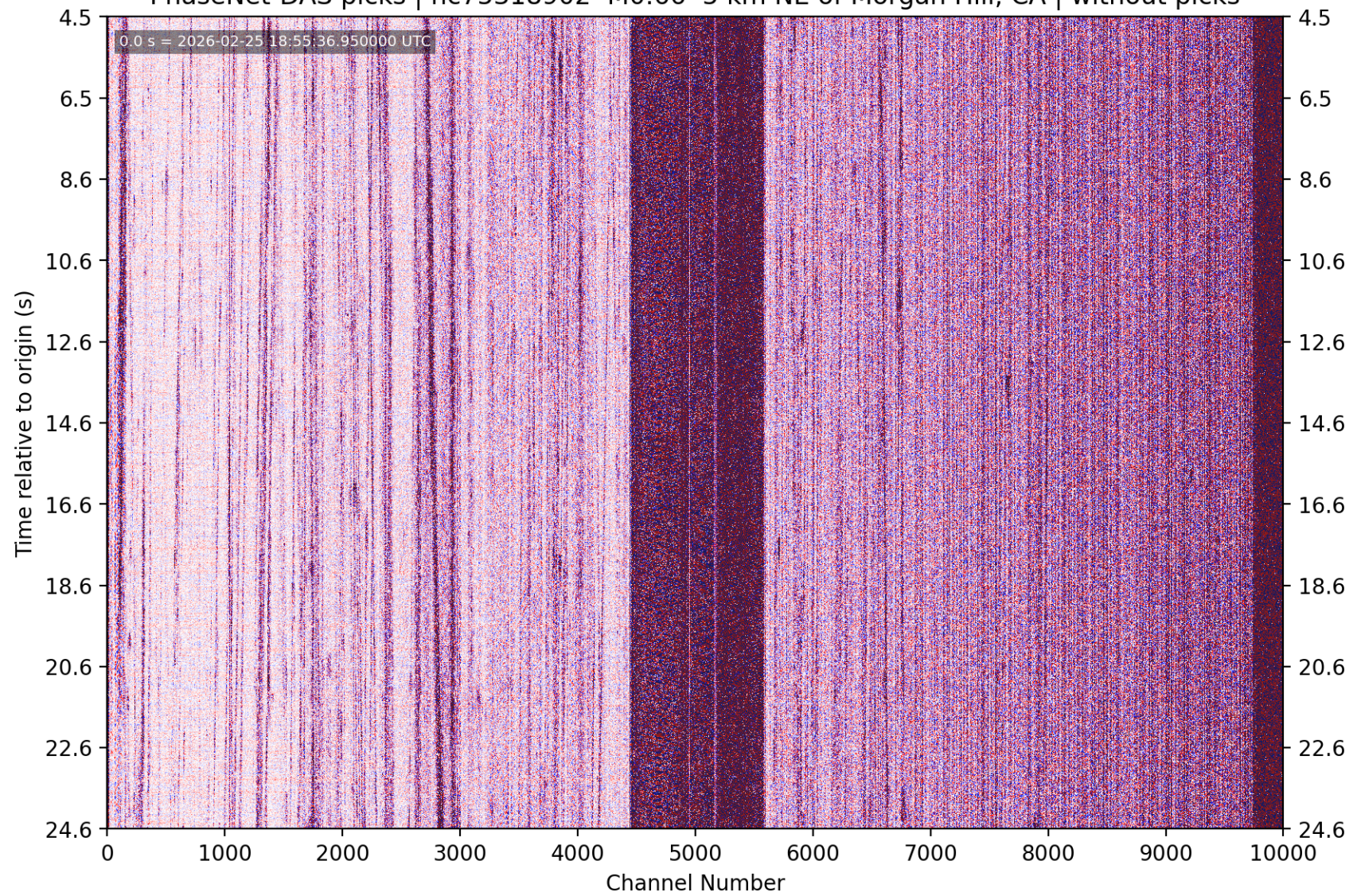
PhaseNet-DAS picks | nc75318902 M0.66 5 km NE of Morgan Hill, CA | without picks
