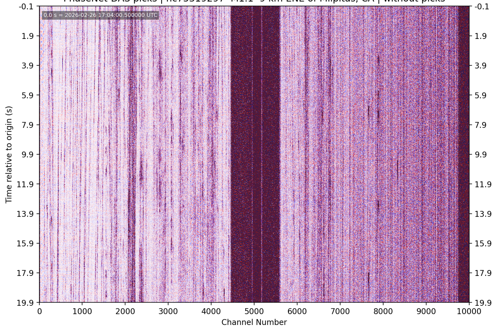
PhaseNet-DAS picks | nc75319297 M1.1 9 km ENE of Milpitas, CA | without picks
