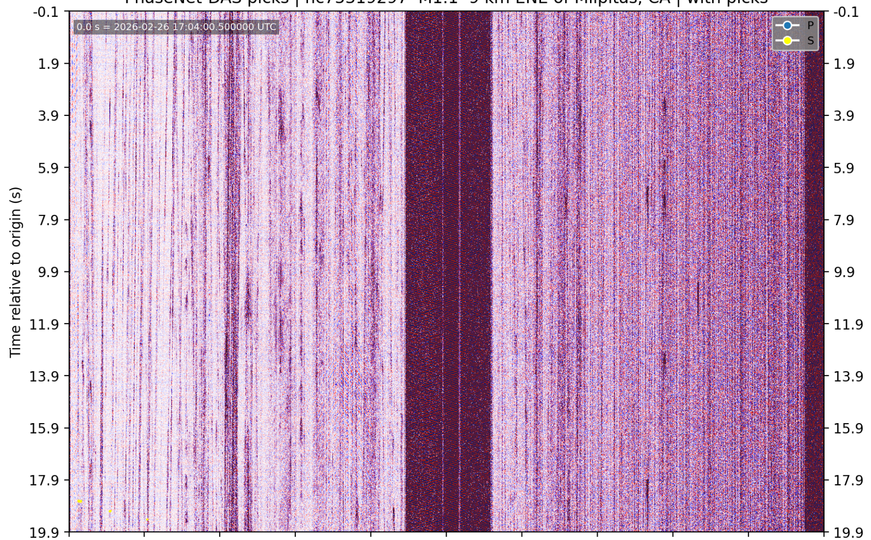
PhaseNet-DAS picks | nc75319297 M1.1 9 km ENE of Milpitas, CA | without picks
