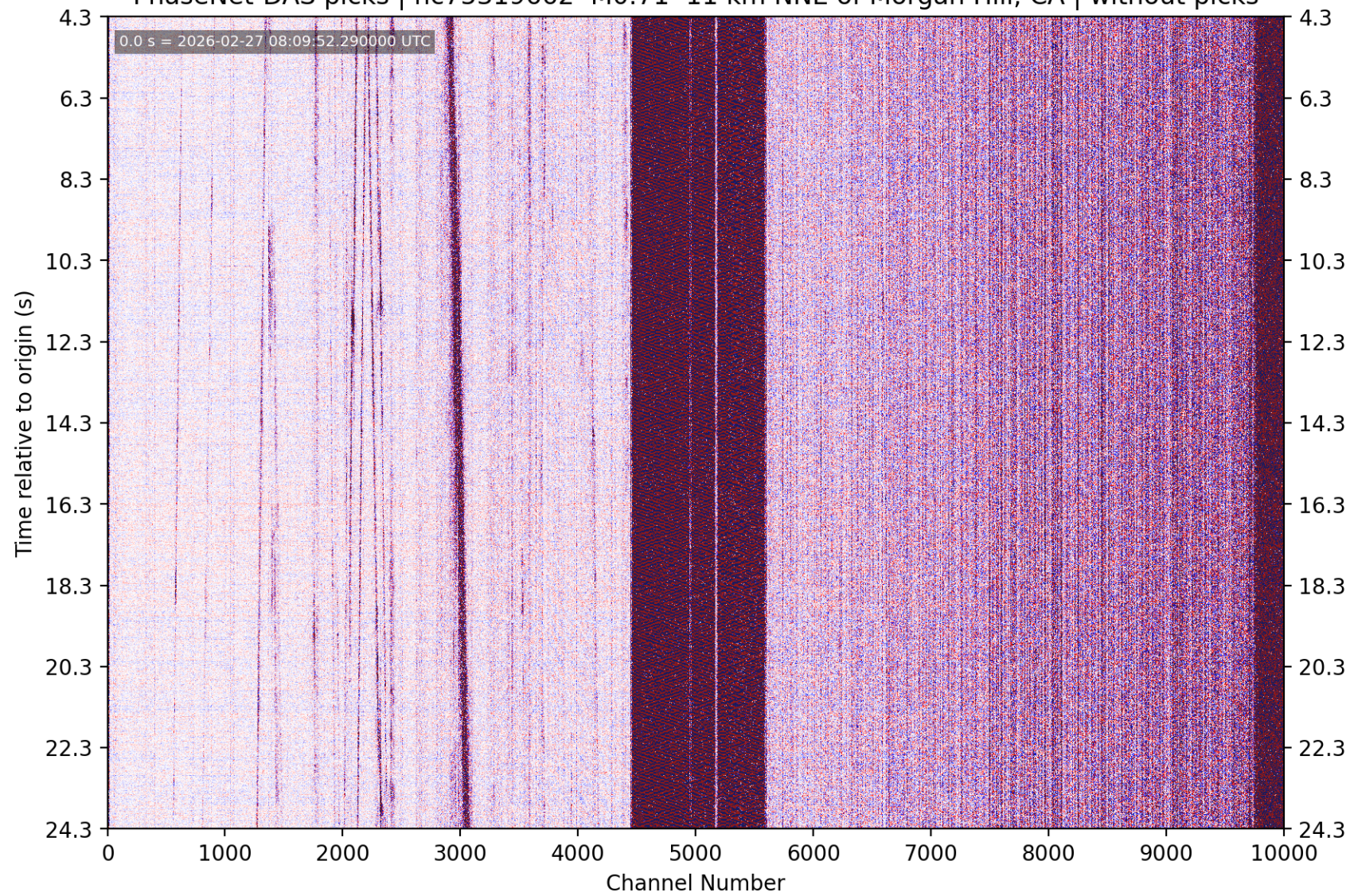
PhaseNet-DAS picks | nc75319662 M0.71 11 km NNE of Morgan Hill, CA | without picks
