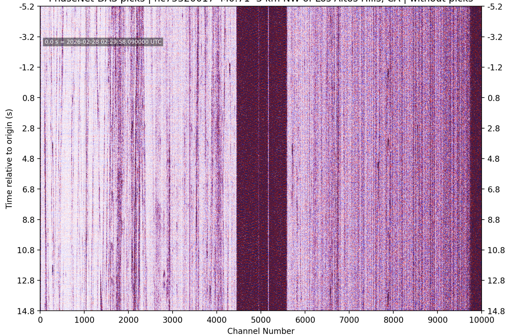
PhaseNet-DAS picks | nc75320017 M0.71 3 km NW of Los Altos Hills, CA | without picks
