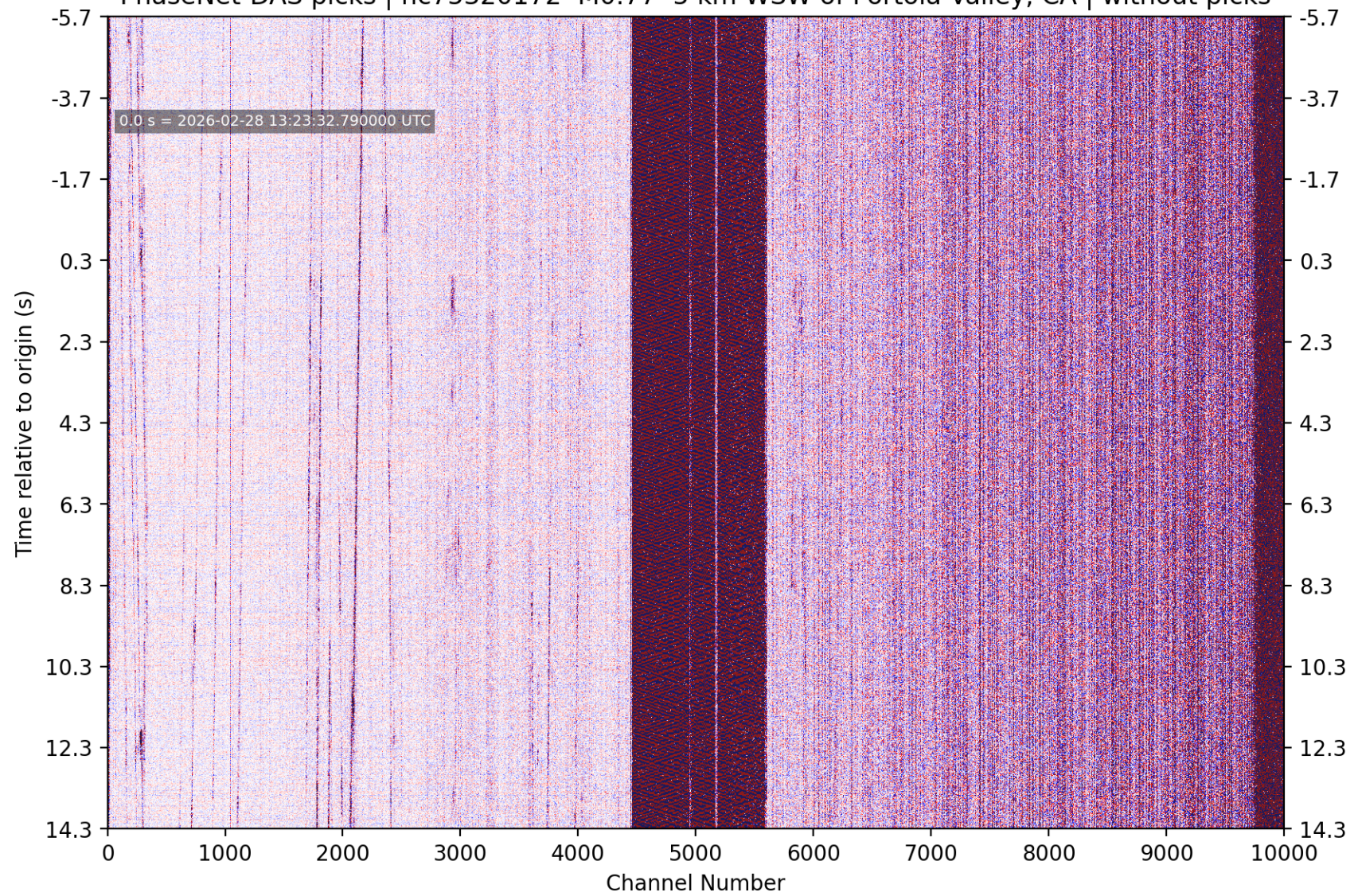
PhaseNet-DAS picks | nc75320172 M0.77 5 km WSW of Portola Valley, CA | without picks
