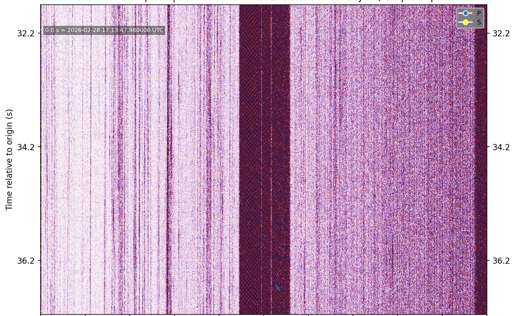
PhaseNet-DAS picks | nc75320267 M0.11 2 km SSW of Loyola, CA | without picks
