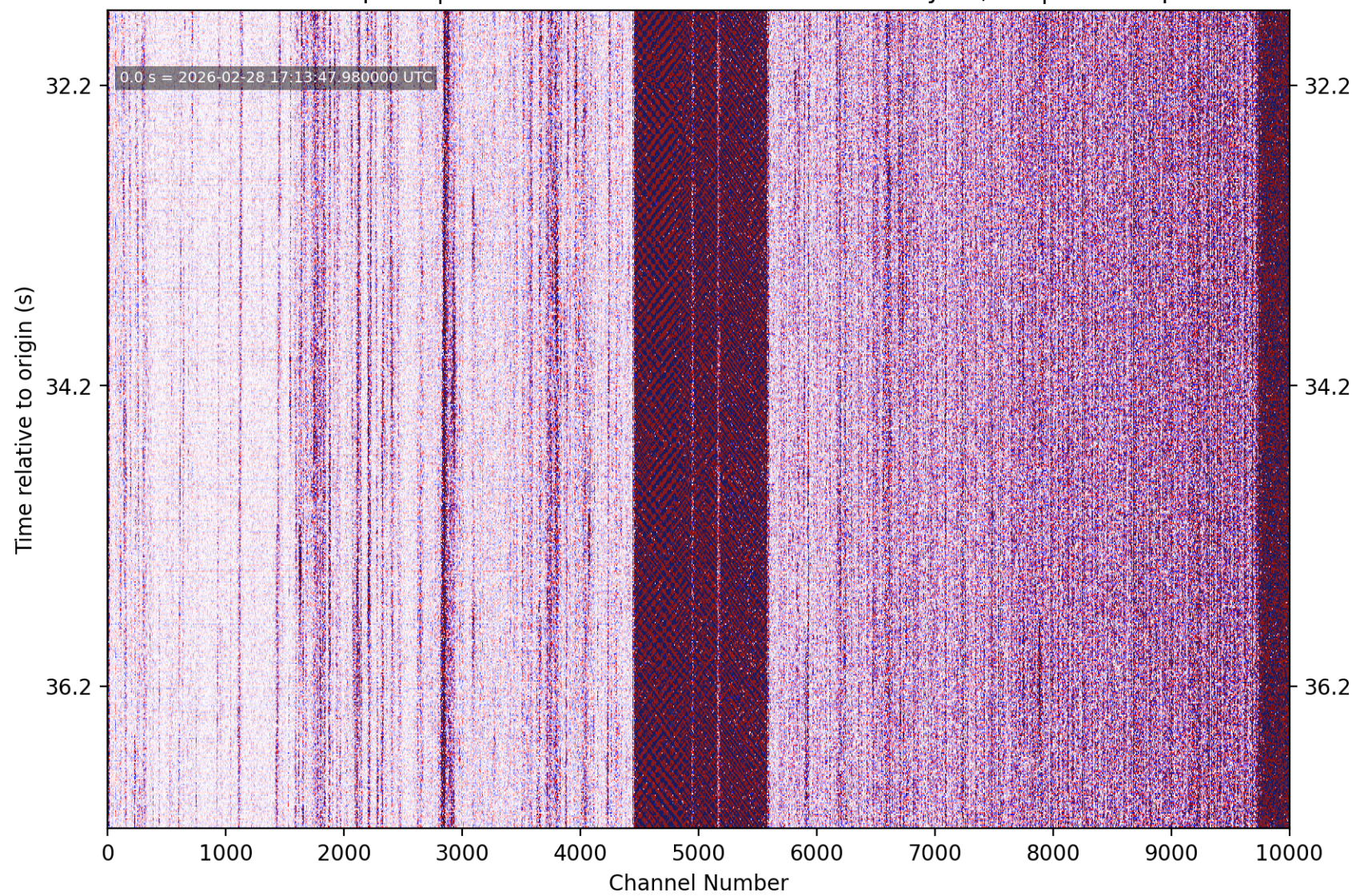
PhaseNet-DAS picks | nc75320267 M0.11 2 km SSW of Loyola, CA | without picks
