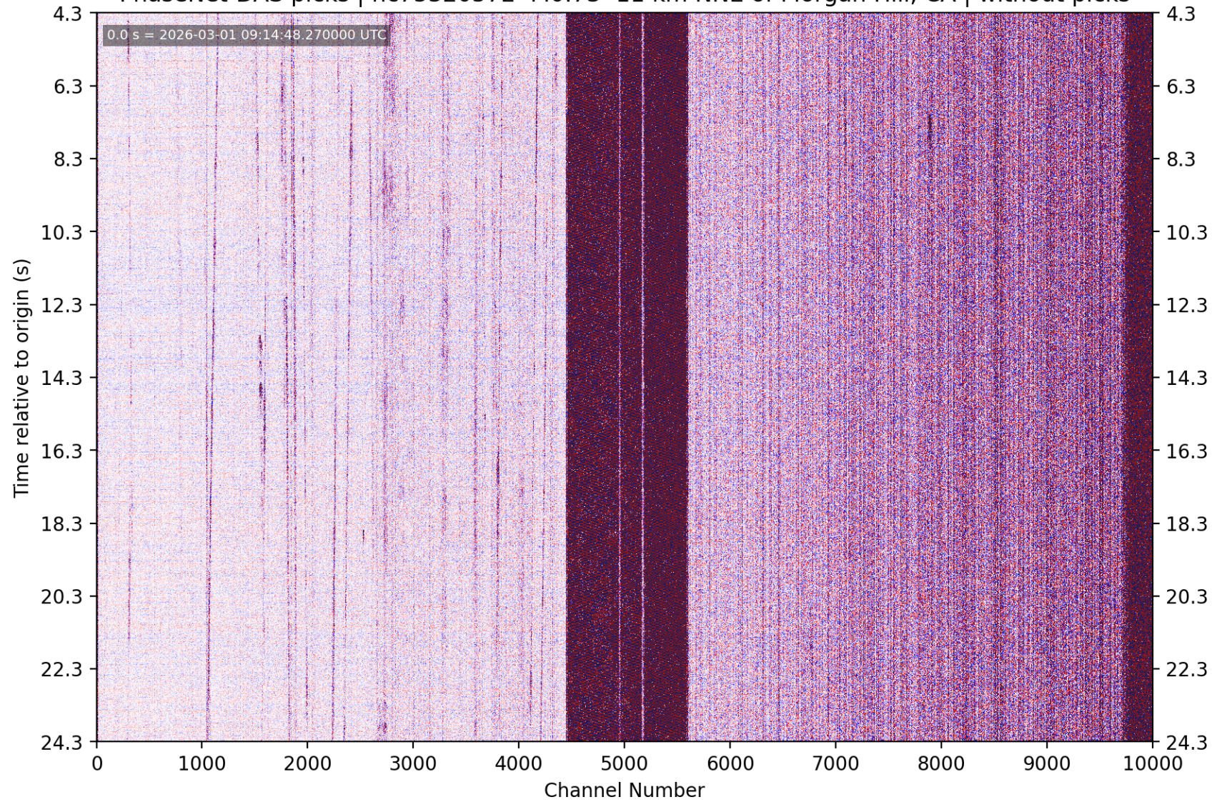
PhaseNet-DAS picks | nc75320572 M0.73 11 km NNE of Morgan Hill, CA | without picks
