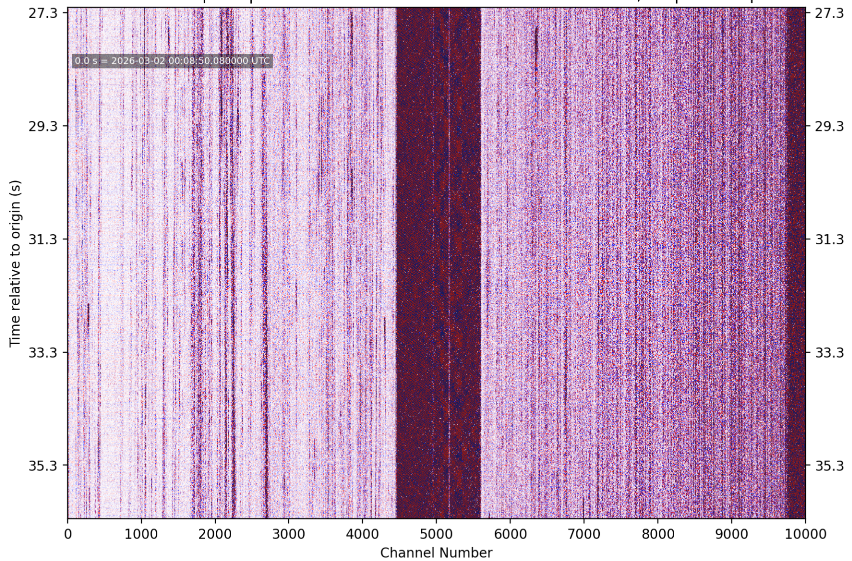
PhaseNet-DAS picks | nc75320977 M0.52 6 km SW of Los Altos Hills, CA | without picks
