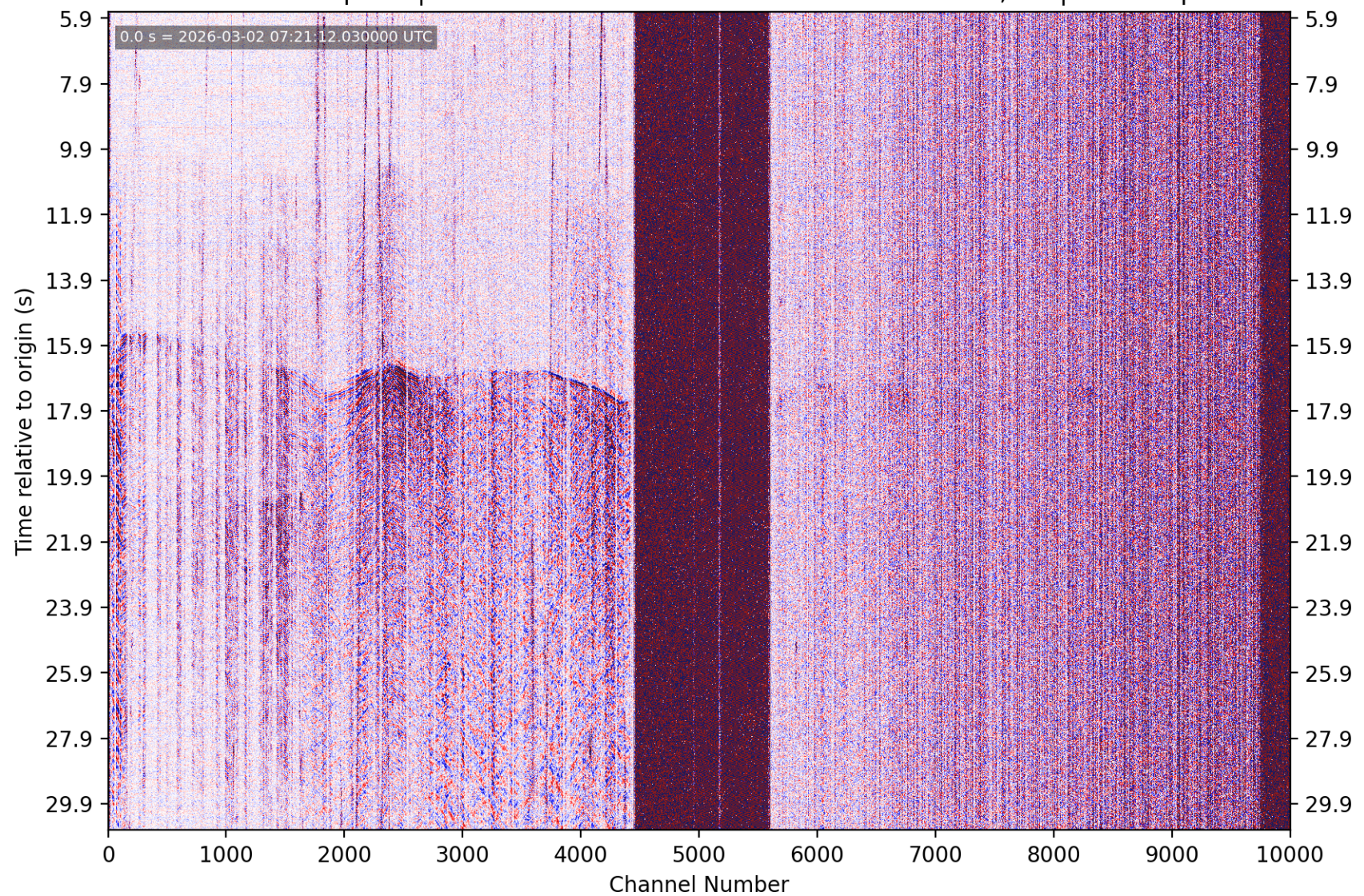
PhaseNet-DAS picks | nc75321147 M3.17 4 km SE of San Ramon, CA | without picks
