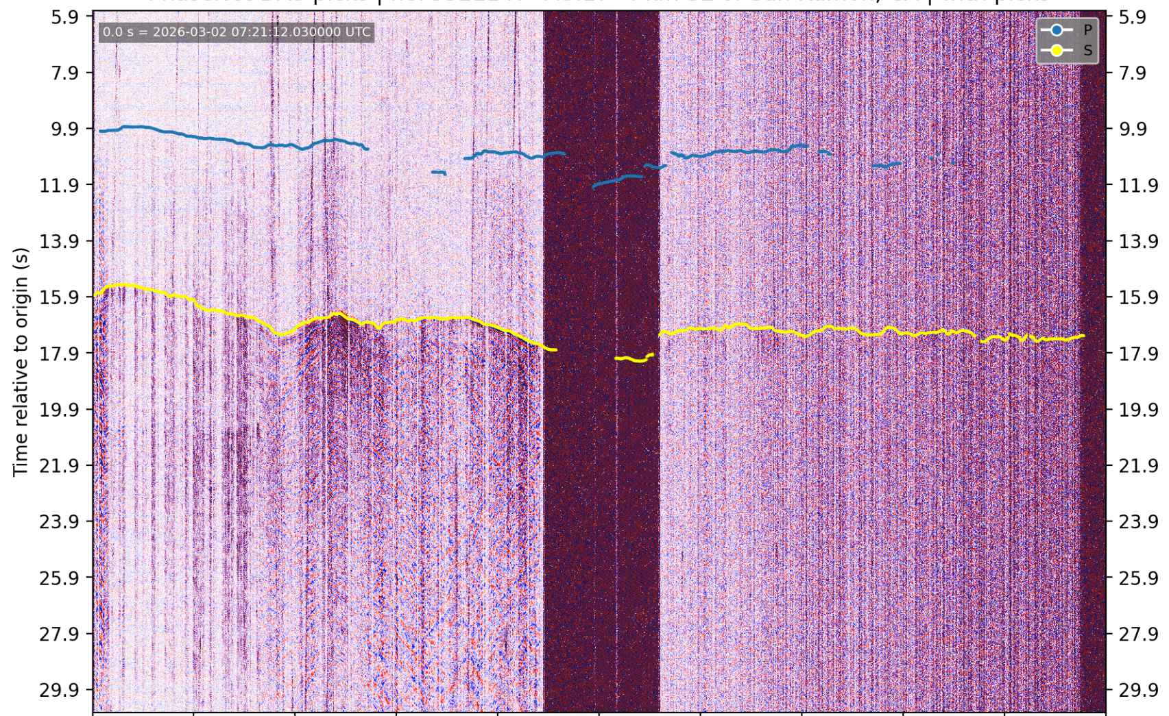
PhaseNet-DAS picks | nc75321147 M3.17 4 km SE of San Ramon, CA | without picks
