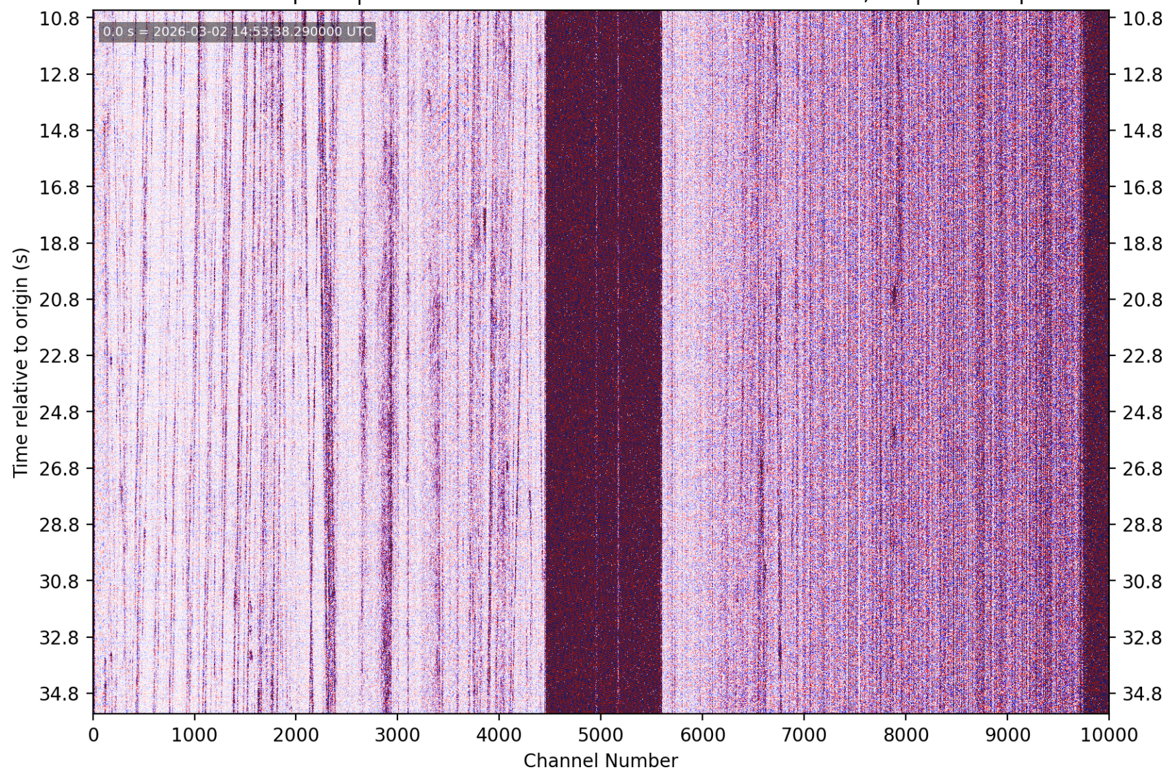
PhaseNet-DAS picks | nc75321372 M1.61 15 km E of Seven Trees, CA | without picks
