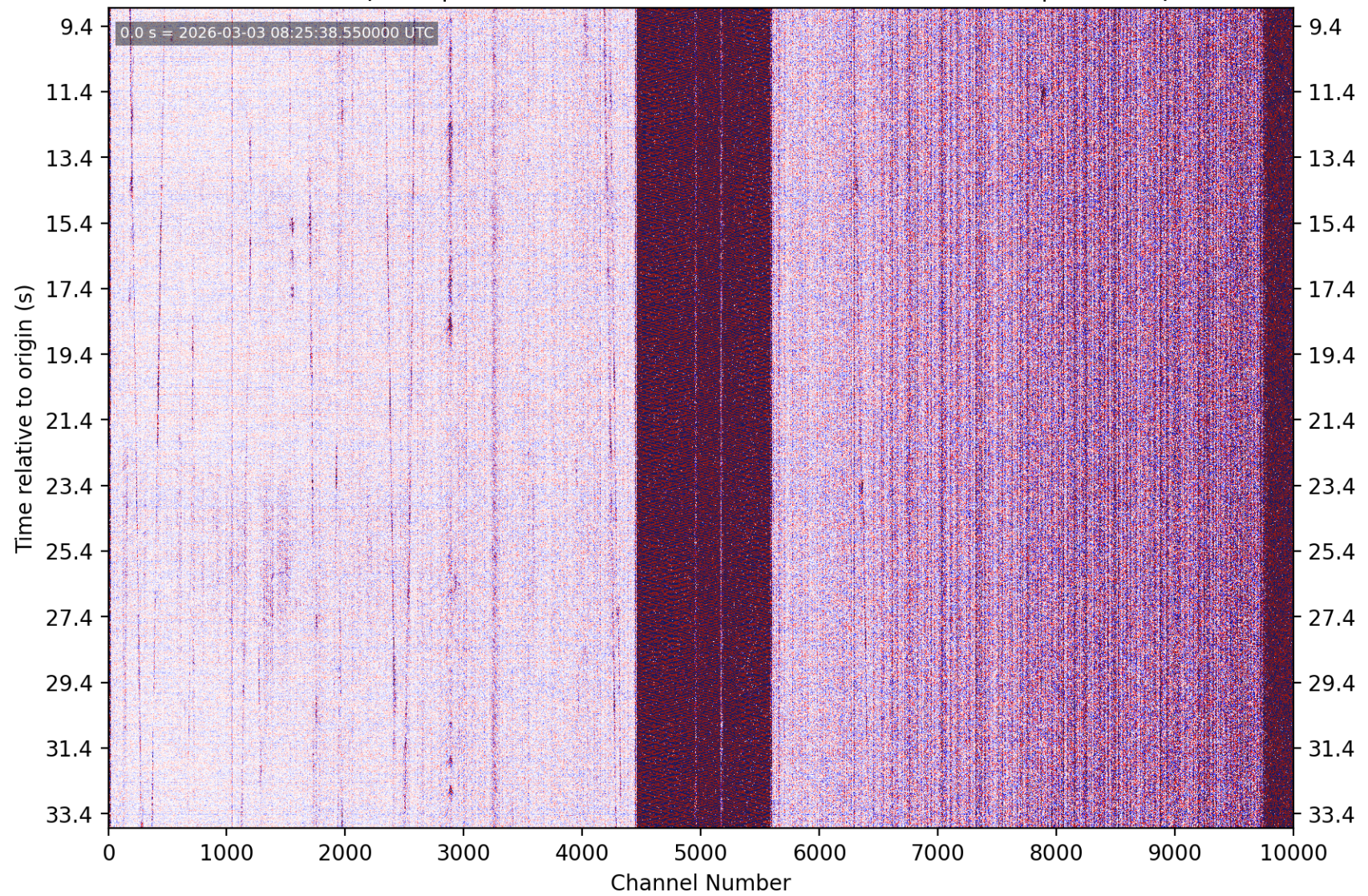
PhaseNet-DAS picks | nc75321807 M1.7 8 km E of Alum Rock, CA | without picks
