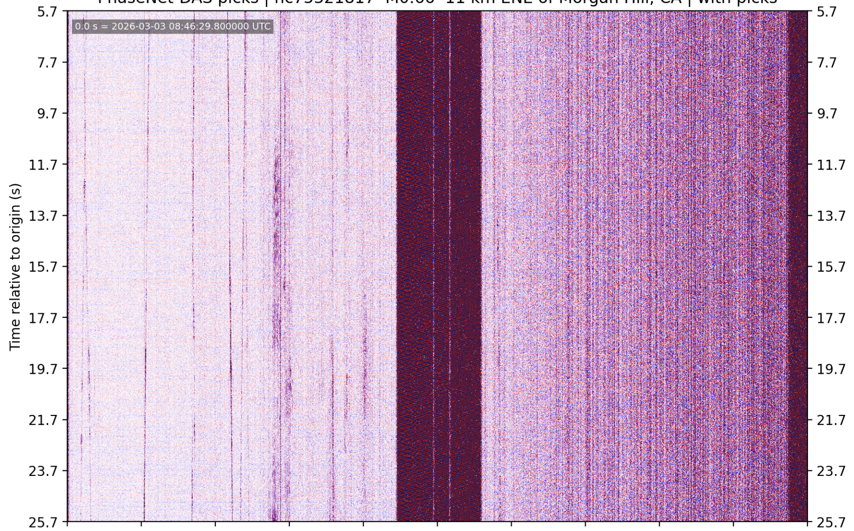
PhaseNet-DAS picks | nc75321817 M0.66 11 km ENE of Morgan Hill, CA | without picks
