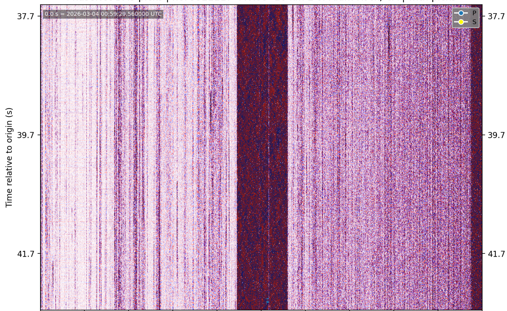
PhaseNet-DAS picks | nc75322217 M0.99 10 km E of Alum Rock, CA | without picks
