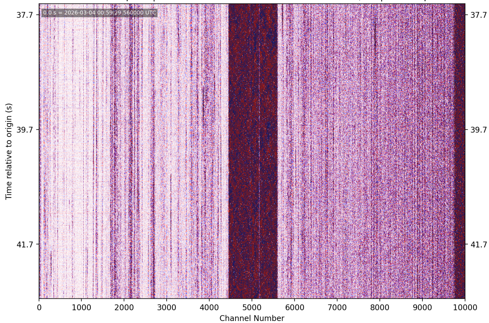
PhaseNet-DAS picks | nc75322217 M0.99 10 km E of Alum Rock, CA | without picks
