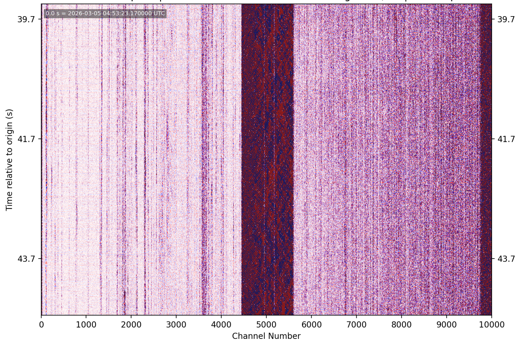
PhaseNet-DAS picks | nc75322767 M0.93 14 km N of Morgan Hill, CA | without picks
