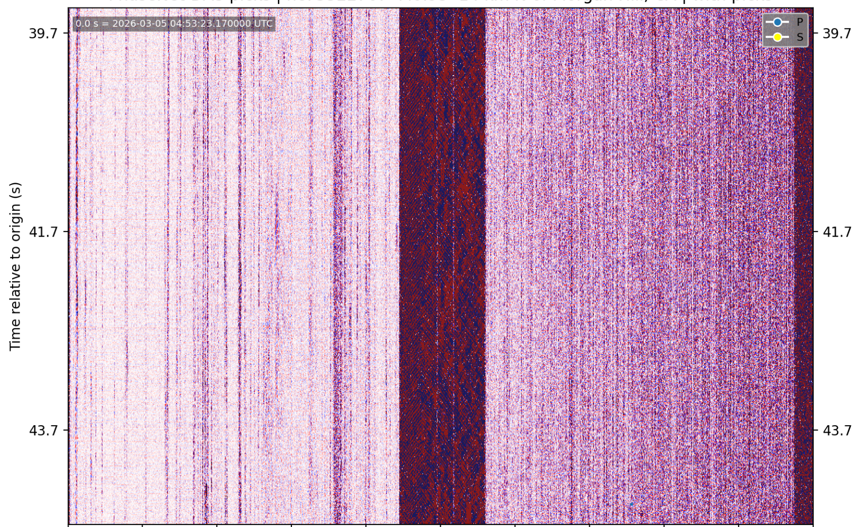
PhaseNet-DAS picks | nc75322767 M0.93 14 km N of Morgan Hill, CA | without picks
