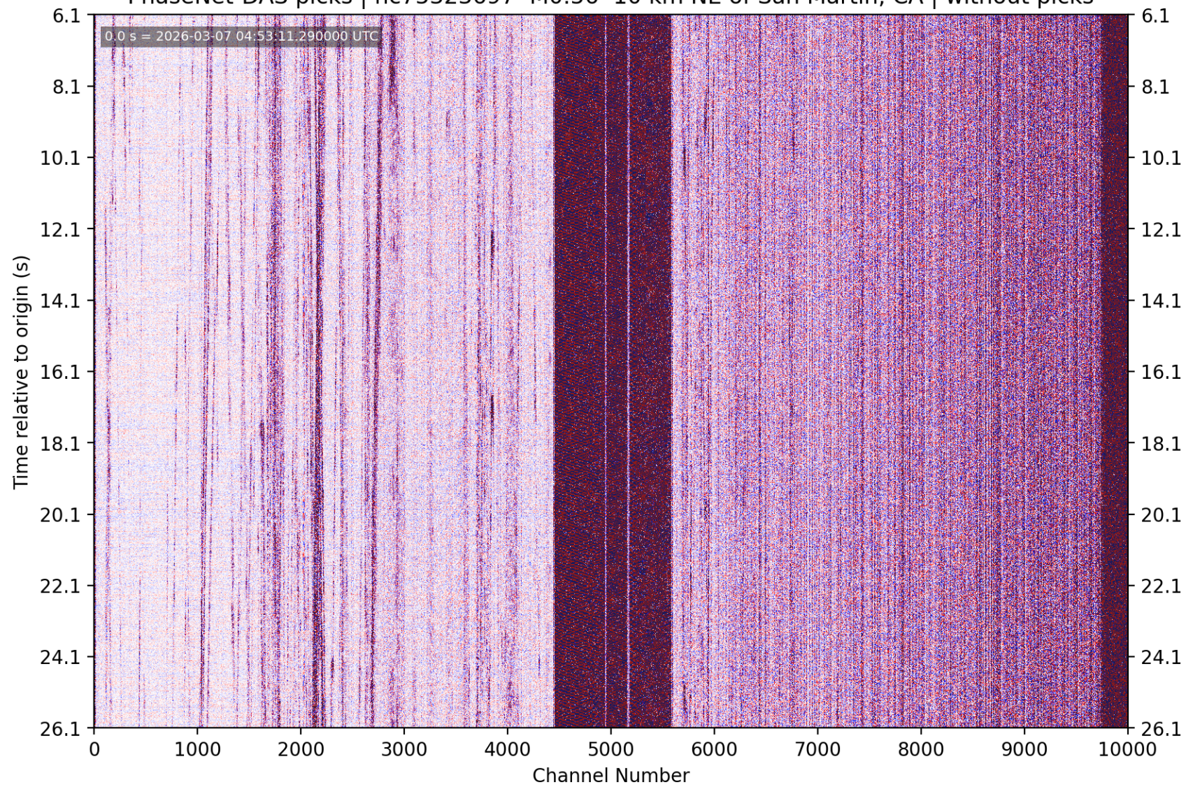
PhaseNet-DAS picks | nc75323697 M0.56 10 km NE of San Martin, CA | without picks
