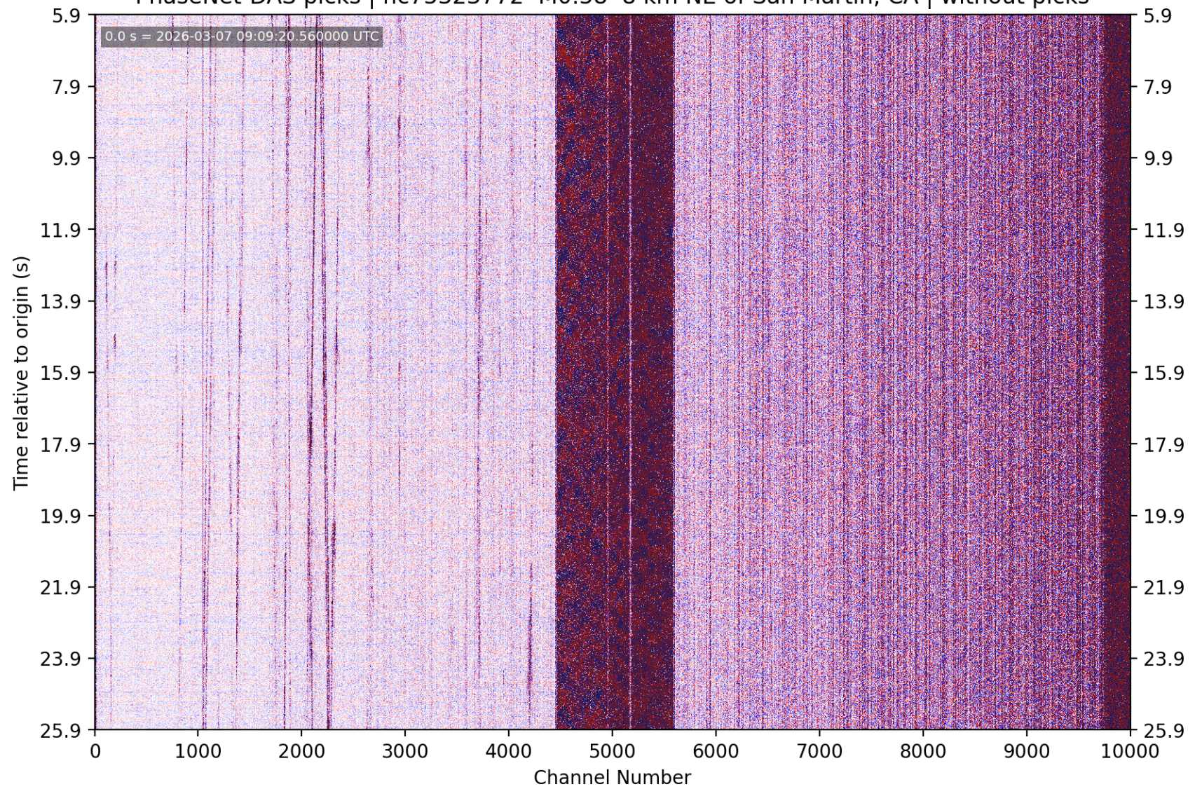
PhaseNet-DAS picks | nc75323772 M0.58 8 km NE of San Martin, CA | without picks
