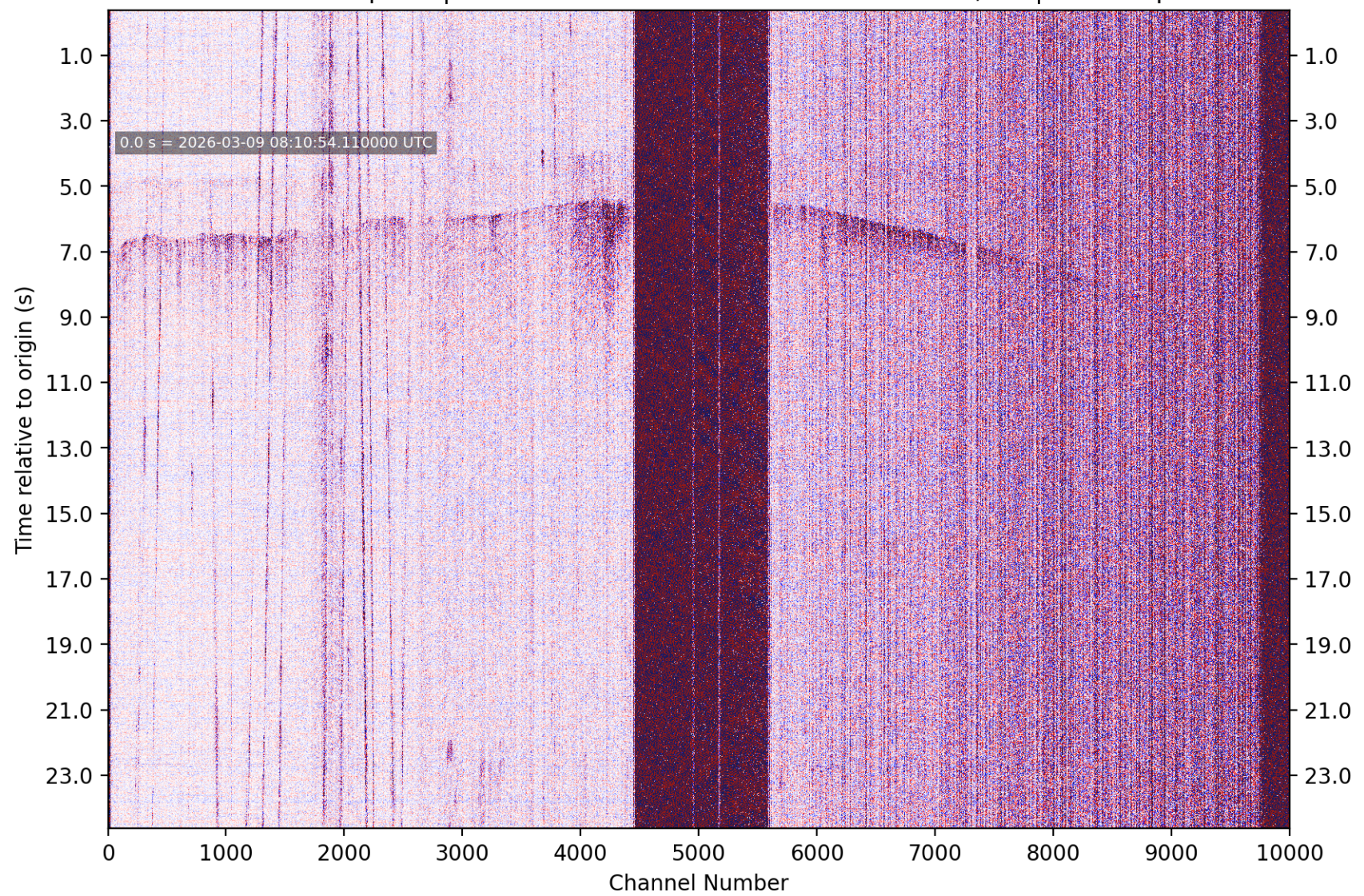
PhaseNet-DAS picks | nc75324877 M1.59 3 km SE of Pacifica, CA | without picks
