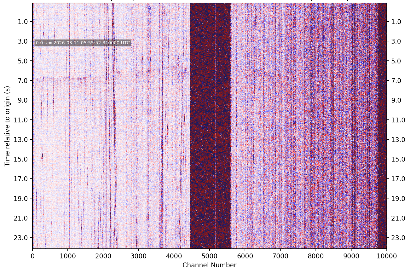
PhaseNet-DAS picks | nc75325737 M1.27 4 km SE of Pacifica, CA | without picks
