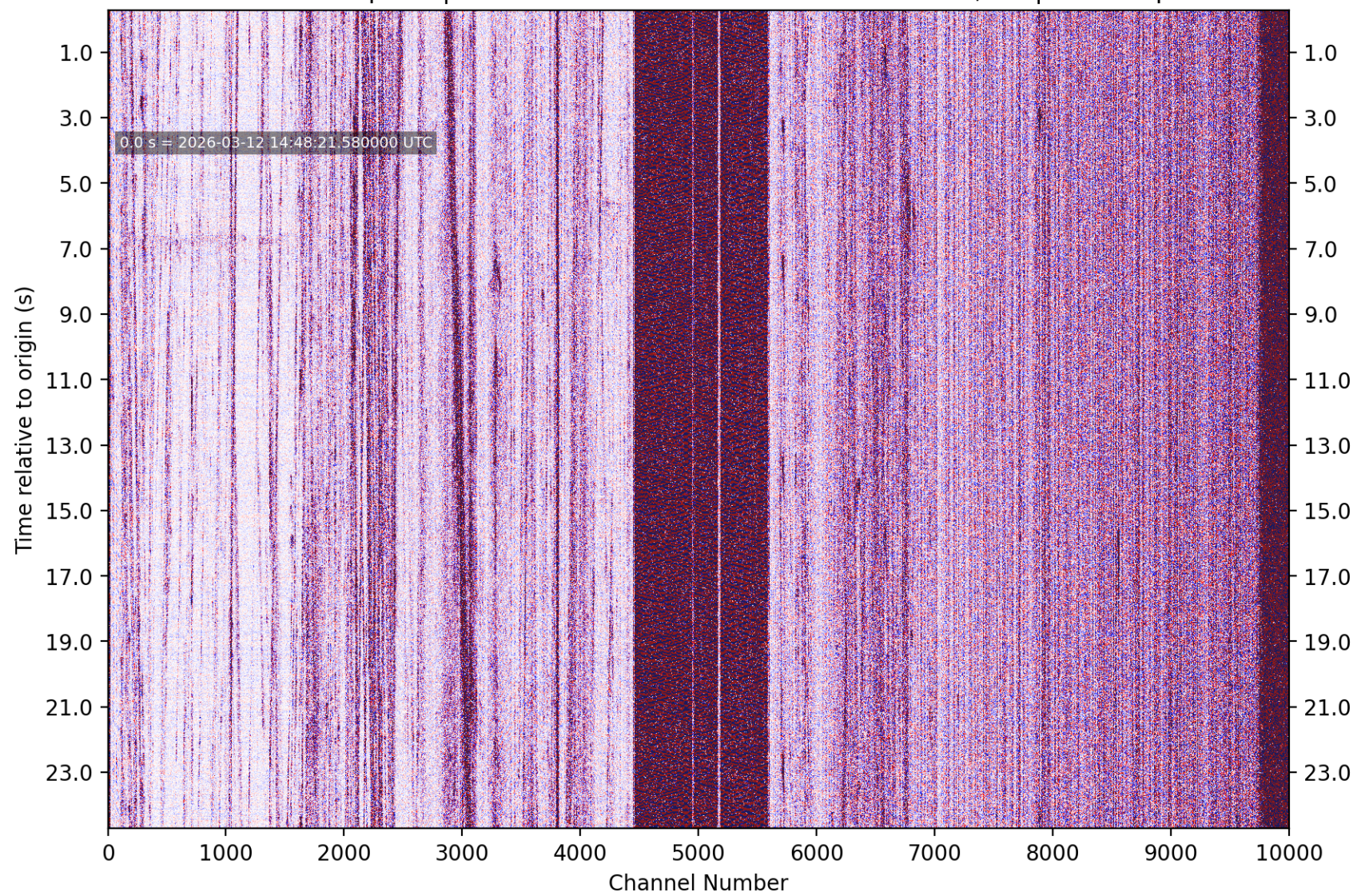
PhaseNet-DAS picks | nc75326502 M0.77 3 km SE of Pacifica, CA | without picks
