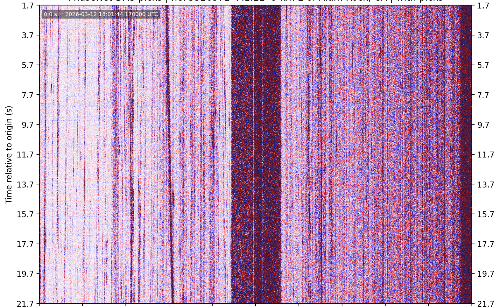
PhaseNet-DAS picks | nc75326572 M1.22 9 km E of Alum Rock, CA | without picks
