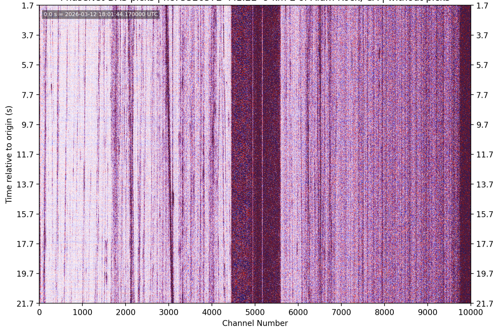
PhaseNet-DAS picks | nc75326572 M1.22 9 km E of Alum Rock, CA | without picks
