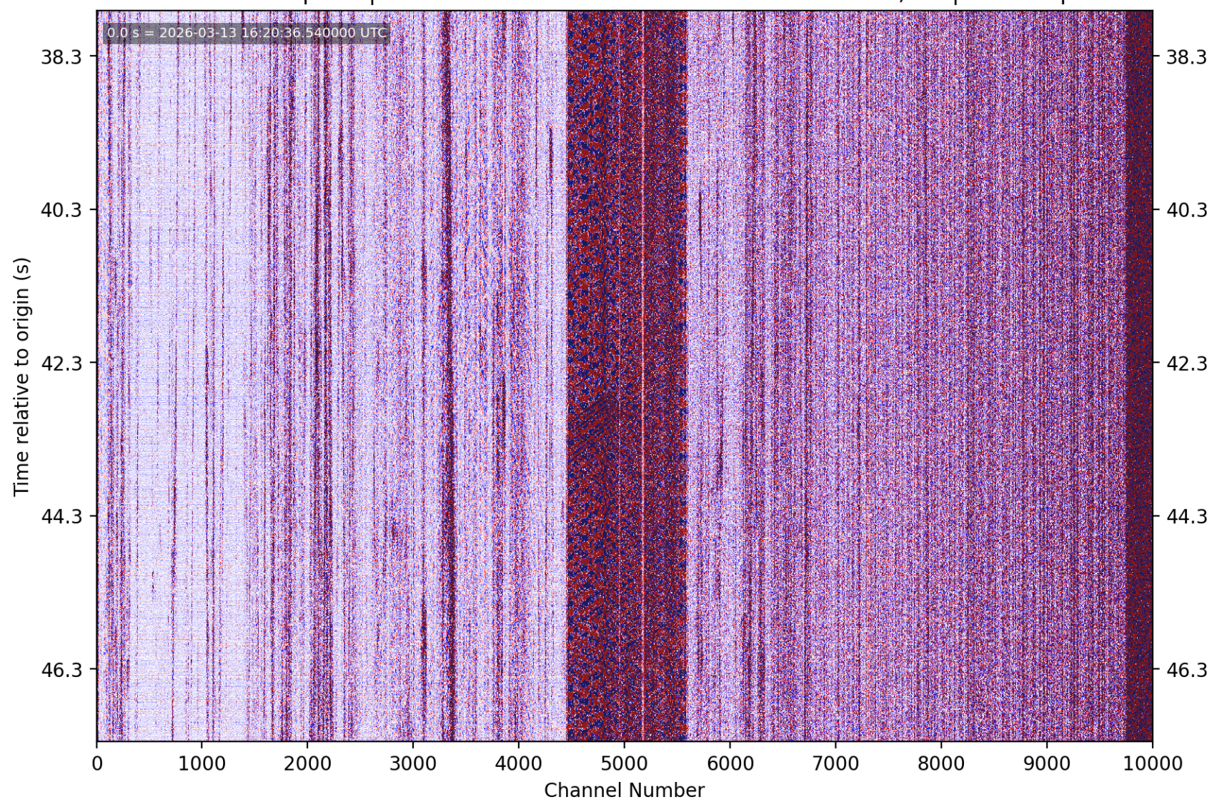
PhaseNet-DAS picks | nc75326952 M0.61 9 km ENE of San Martin, CA | without picks
